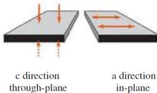
Illustration from Ex. 2005 ¶ 81 showing “c-direction” through plane and “a-direction” in-plane thermal conductivity.
