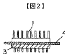
Fig. 2 of Inoue (Ex. 1016) showing carbonaceous sheet 4 and semiconductor (heat source) 3.
