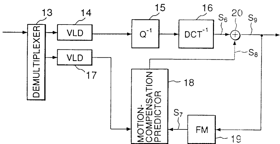
FIG.2 PRIOR ART
