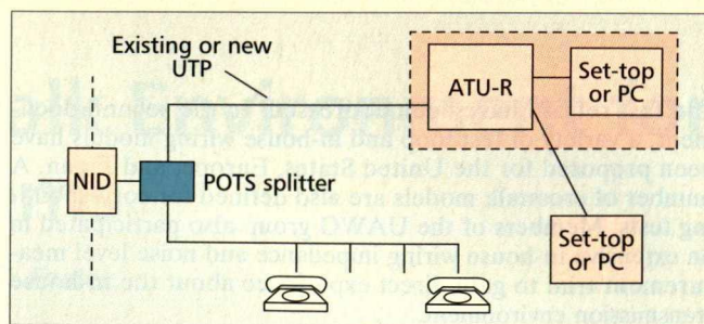
■ Figure 3. An ATU-R with a separate POTS splitter.
