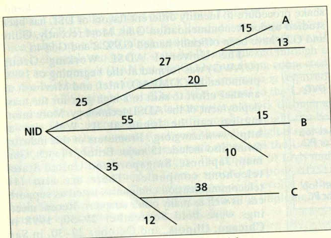
■ Figure 5. A random in-house wiring model.
