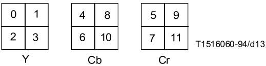
Figure 6-12 – 4:4:4 Macroblock structure
