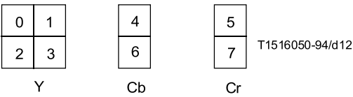
Figure 6-11 – 4:2:2 Macroblock structure
