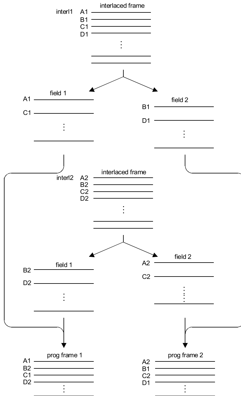
Figure D.4 – Two interlace to progressive conversion
