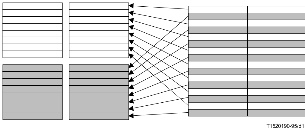
Figure 6-14 – Luminance macroblock structure in field DCT coding
