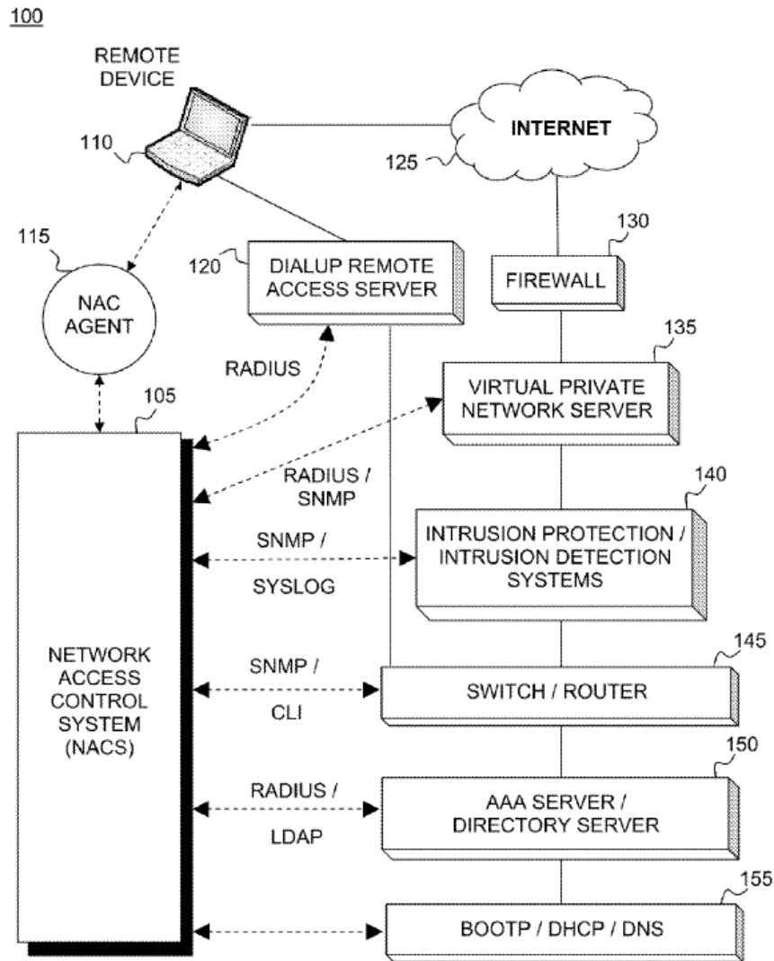
(NETWORK ACCESS CONTROL ARCHITECTURE) FIG. 1
