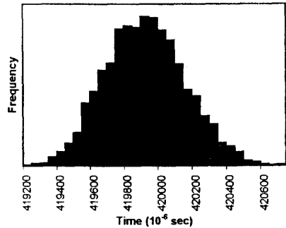
FIGURE 2: RSAREF Modular Exponentiation Times
