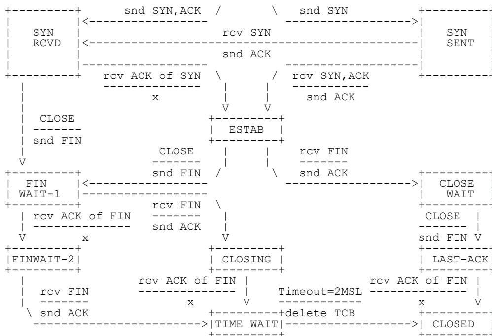
TCP Connection State Diagram Figure 6.
