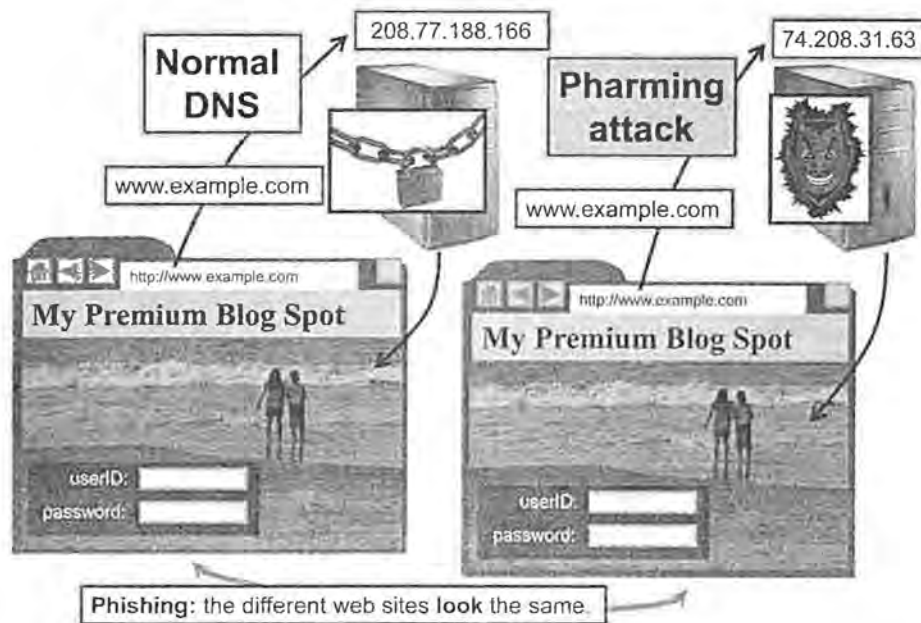
Figure 6.5: A pharming attack that maps a domain name to a malicious server, which then performs a phishing attack by delivering a web page that looks the same as the real one, to trick people into entering their userIDs and passwords. (Image by Karen Goodrich; used with permission.)
