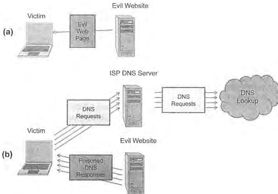
Figure 6.8: A DNS cache poisoning attack against a client: (a) On visiting a malicious web site, the victim views a page containing many images, each causing a separate DNS request to be made to a nonexistent subdomain of the domain that is to be poisoned. (b) The malicious web server sends guessed responses to each of these requests. On a successful guess, the client's DNS cache will be poisoned.
