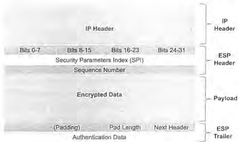
Figure 6.16: The ESP header.
