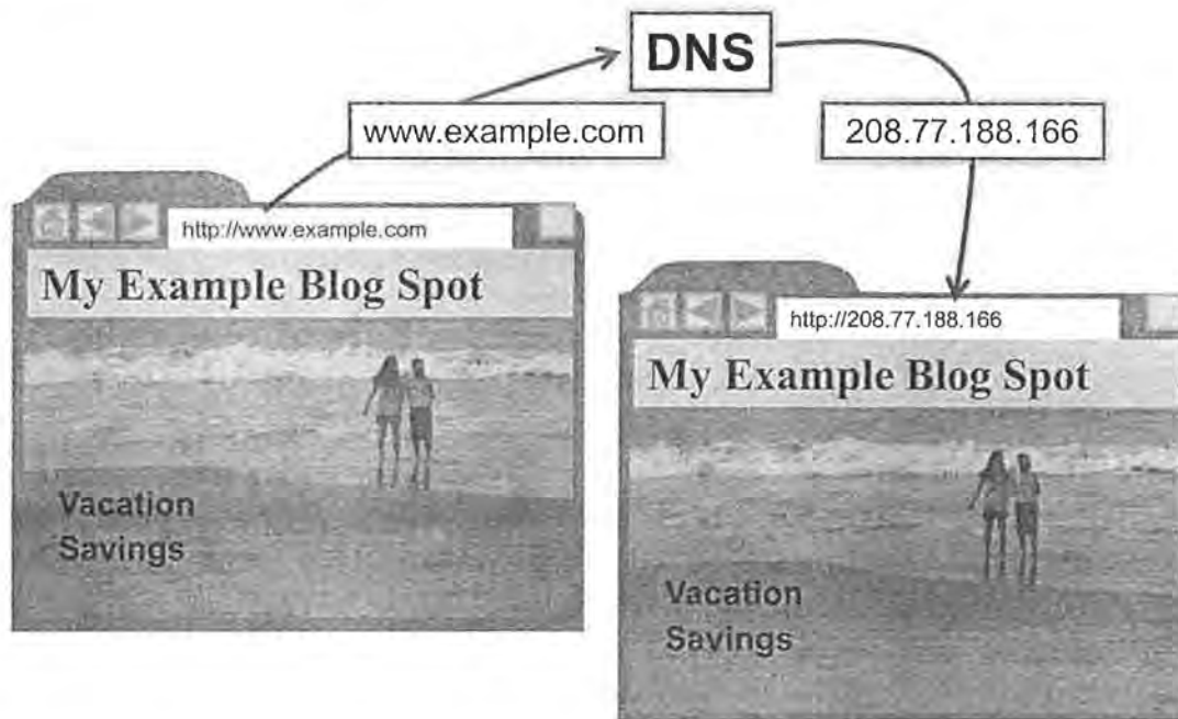
Figure 6.1: The DNS protocol performs a lookup for domain name www.example.com to find the IP address associated with this domain. (Image by Karen Goodrich; used with permission.)
