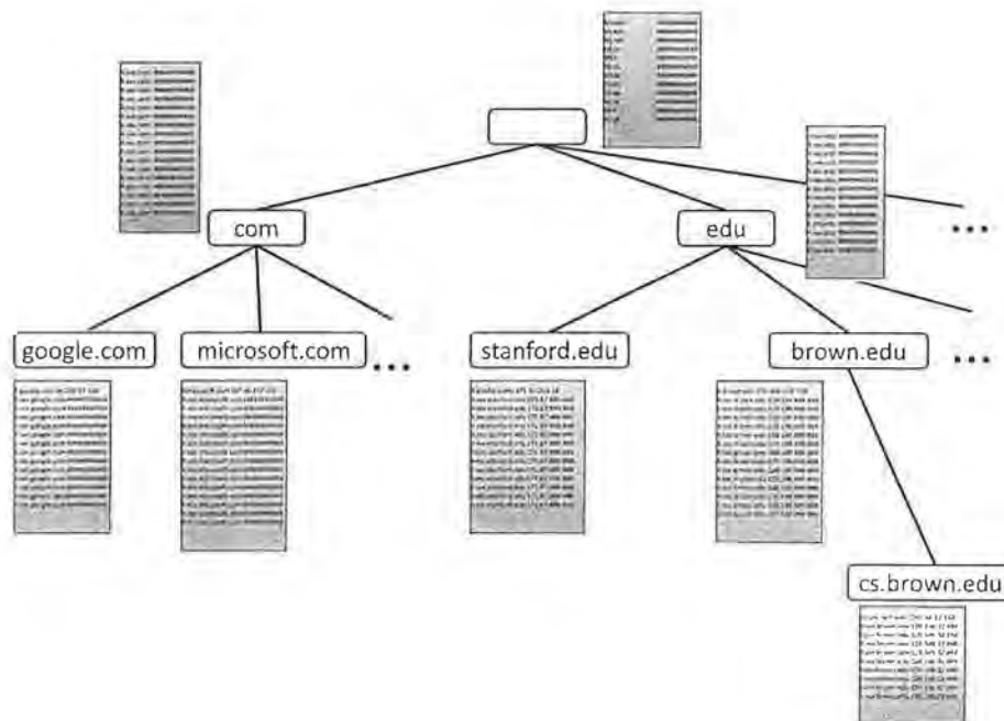
Figure 6.2: The hierarchical organization of authoritative name servers. Each name server stores a collection of records, each providing the address of a domain or a reference to an authoritative name server for that domain.
