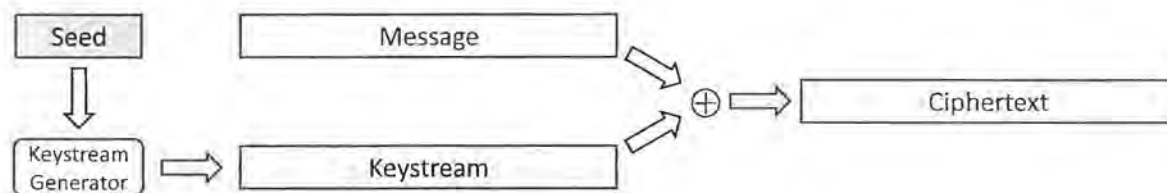
Figure 6.24: Encryption with a stream cipher.
