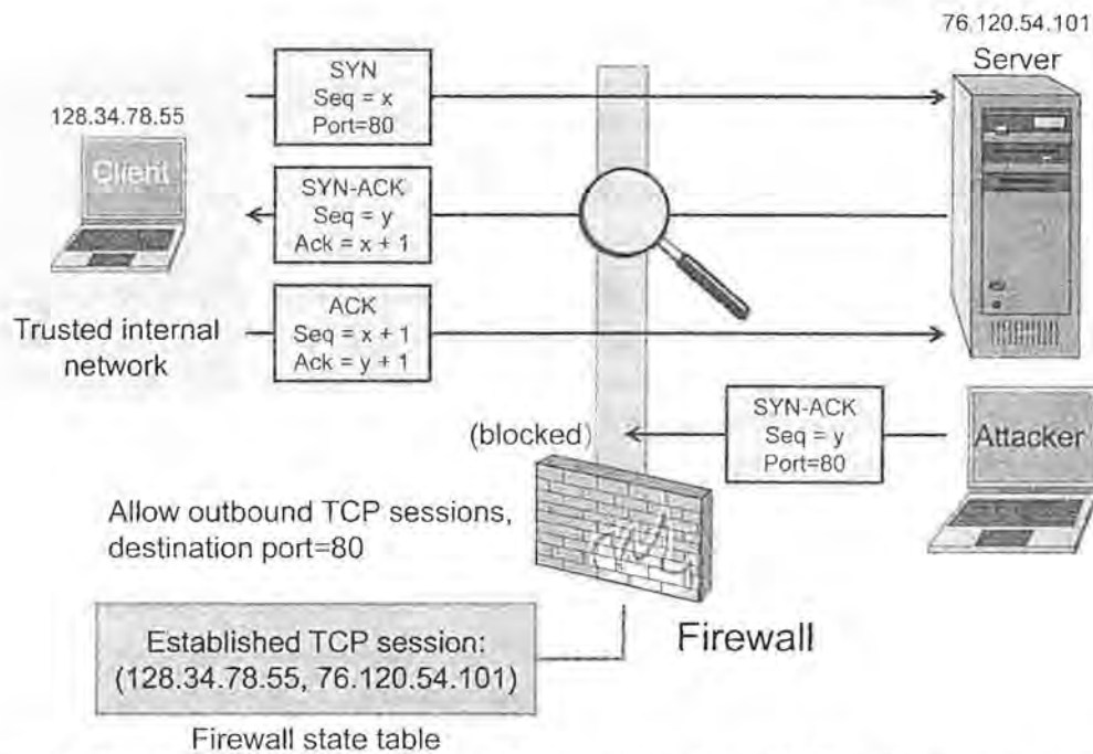
Figure 6.13: A stateful firewall configured to allow TCP web sessions (port 80) with a request coming from inside the trusted internal network.
