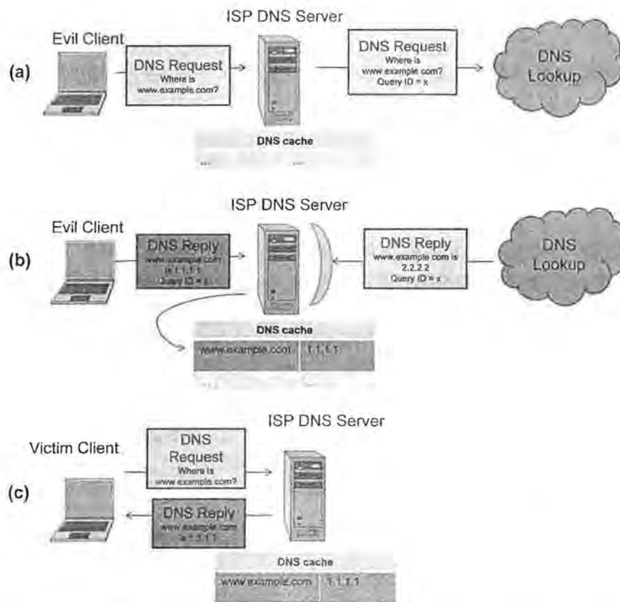
Figure 6.6: A DNS cache poisoning attack: (a) First, the attacker sends a DNS request for the domain he wishes to poison. The ISP DNS server checks its cache and queries root name servers for the domain. (b) The attacker sends a corresponding reply for his own request, guessing the transaction ID. If he successfully guesses the random query ID chosen by the ISP DNS server, the response will be cached. (c) Any clients of the ISP DNS server issuing DNS requests for the poisoned domain will be redirected to the attacker's IP address.
