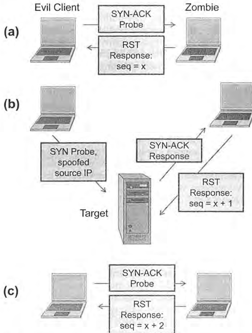
Figure 6.21: An idle scan: (a) The attacker probes a zombie with predictable sequence numbers. (b) The attacker sends a spoofed TCP packet to the target. (c) The attacker checks the state of the port by probing the zombie again.
