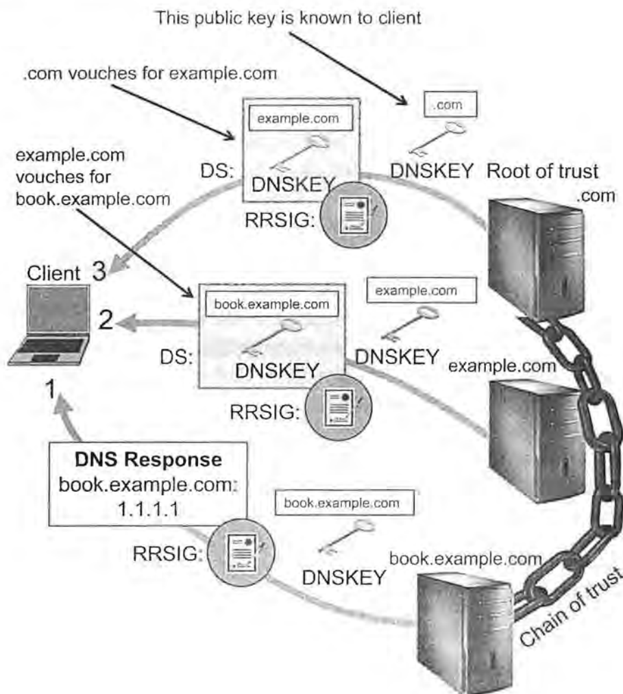
Figure 6.9: A DNSSEC response and the chain of trust that validates it. In this case, book.example.com returns a signed DNS response along with its public key, example.com sends its public key and a signed DS record validating the public key of book.example.com , and .com sends its public key and a signed DS record validating the public key of example.com . The client can trust this chain, since it knows the public key of .com .
