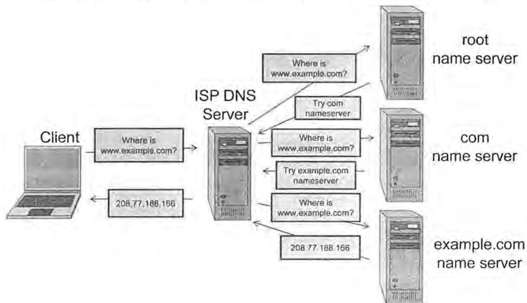
Figure 6.3: A typical execution of a DNS query. The client machine queries a designated name server, such as a name server of its service provider. The designated name server in turn queries a root name server, then a top-level domain name server, and finally the authoritative name server for the requested domain. Once the intermediate name server resolves the domain name, it forwards the answer to the client machine.
