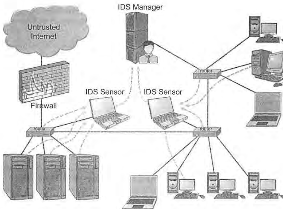
Figure 6.17: A local-area network monitored by an intrusion detection system (IDS). Solid lines depict network connections and gray dashed lines depict data reporting responsibilities. Routers and selected computers report to IDS sensors, which in turn report to the IDS manager.
