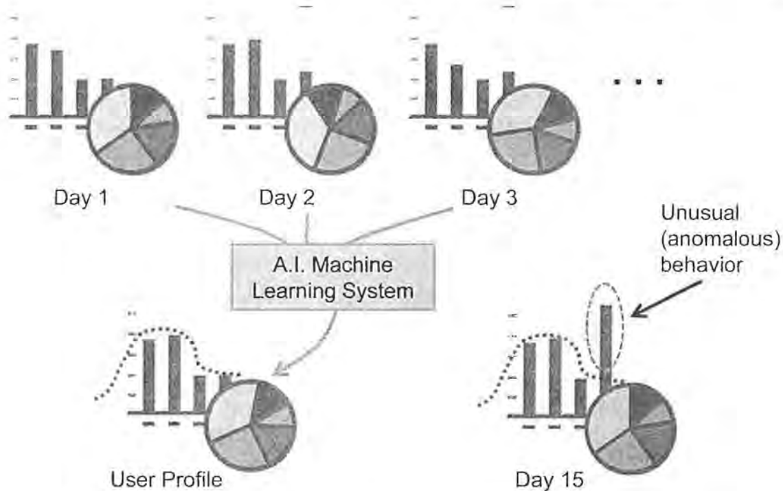
Figure 6.19: How a statistical intrusion detection system works. Statistics about a user are gathered over a sequence of days, and a user profile is determined based on typical behaviors, as defined by an artificial-intelligence machine learning system. Then, on a day when one of the measures is highly unusual compared to the user profile, an alarm would be sounded.
