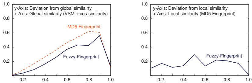
Fig. 4. Classification characteristics within the above plagiarism analysis task. Left: Similarity deviation of fingerprinting compared to the cosine similarity under the vector space model. Right: Similarity deviation of fuzzy-fingerprinting compared to optimum MD5 fingerprinting.
