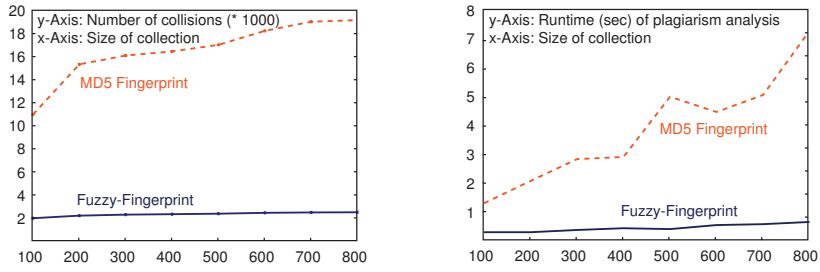
Fig. 3. Runtime performance of a plagiarism analysis task: 50 documents are compared to different subsets of the RFC collection. The figures show the runtime expressed in the number of fingerprint collisions (left) as well as in seconds (right).
