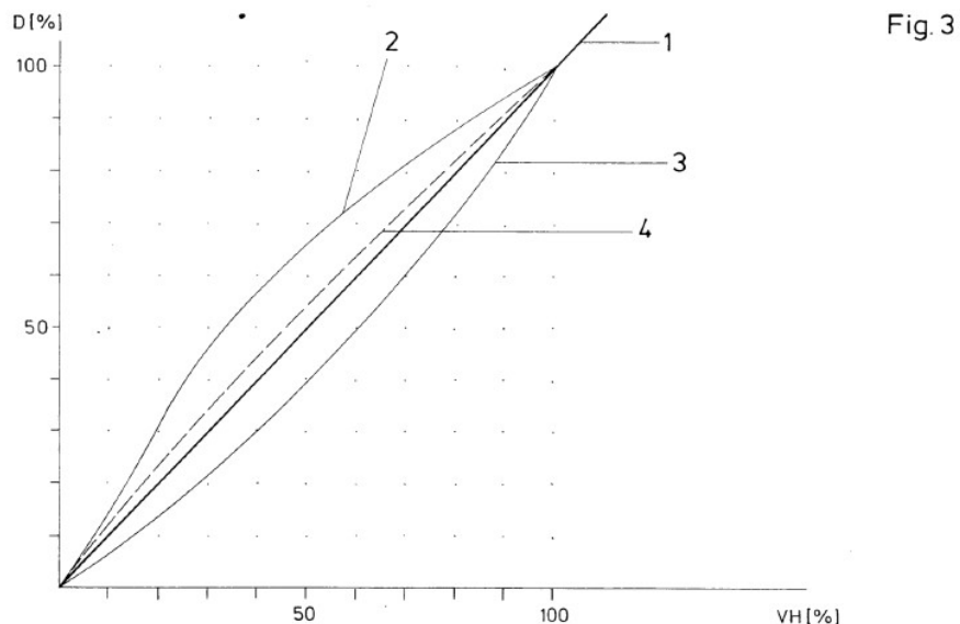
Figure 3 of Erdmann showing “a schematic illustration of a first set of characteristic curves consisting of the valve stroke/flow rate characteristic curve of the control valve.” Ex. 1008, 8:32–34; Pet. 81–82.
