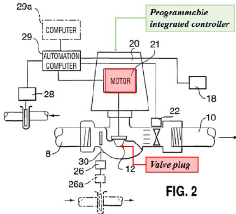
Petitioner's annotated version of Figure 2 showing valve 30, controller 20, valve motor 21, and valve plug 12. Pet. 31
