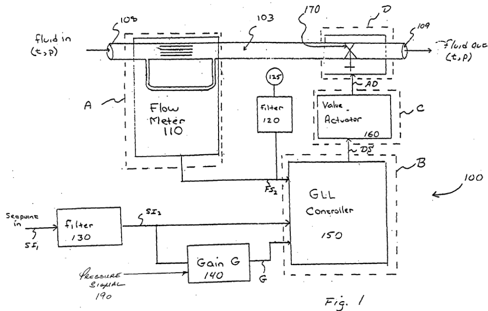
Figure 1 of Lull (Ex. 1009) is a schematic block diagram of a mass flow controller 100 that includes flow meter 110, GLL (Gain/Lead/Lag) controller 150, valve actuator 160, and valve 170. Id. ¶ 106.
