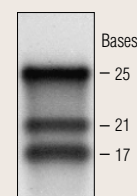
microRNA Marker (ssRNA) 60 ng/lane 12% polyacrylamide-urea gel
