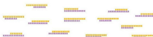
Figure 2 Fragmented DNA
