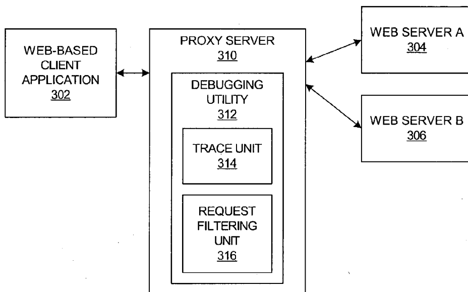
FIG. 3 (PRIOR ART)
