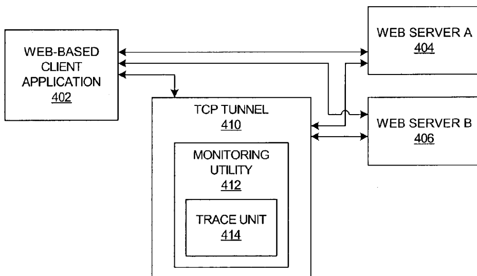
FIG. 4 (PRIOR ART)
