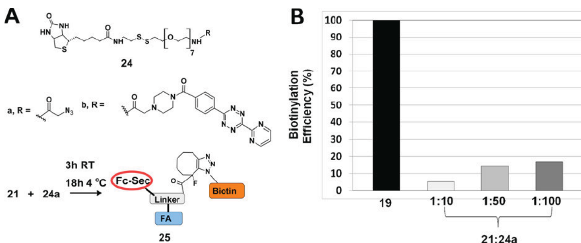
Figure 5. Biotinylation reagents 24a and 24b used to “arm” Fc Sec proteins 21–23. (A) SPAAC reaction of Fc Sec protein 21 (5 \mu g/mL) with biotin azide 24a. Reactions were conducted at room temperature (3 h) then overnight (4 ^\circ C) in PBS, pH 7.4. (B) SPAAC reaction of 21 with 24a. Protein 21 was mixed with 10, 50, and 100 fold excess 24a as described above and then incubated with FR(+) HeLa cells. The cells were stained with PE coupled avidin and then analyzed by flow cytometry. The upper limit of biotinylation is defined as the mean fluorescence intensity (MFI) exhibited by 19. Biotinylation efficiency is expressed as 100(\text{MFI}_{25}/\text{MFI}_{19}) .
