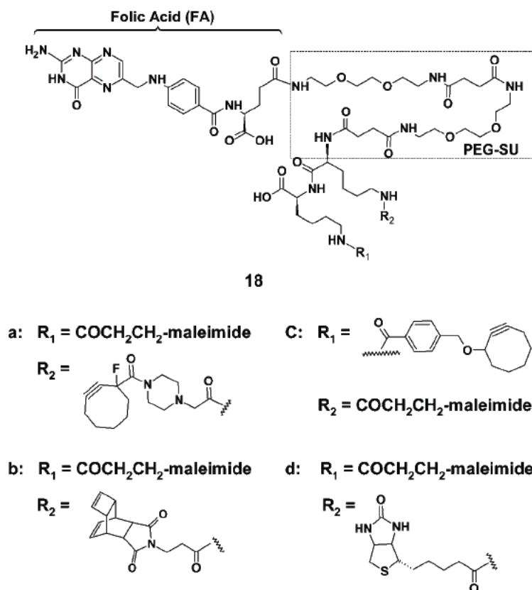
Figure 3. Bifunctional FA conjugates 18a–d for Fc Sec programming.
