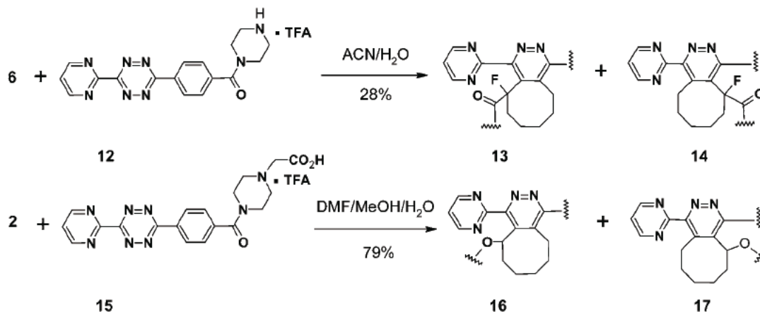
Scheme 3. [4 + 2] Cycloaddition Reactions of Free 6 and 2 with Tetrazines 12 and 15, Respectively
