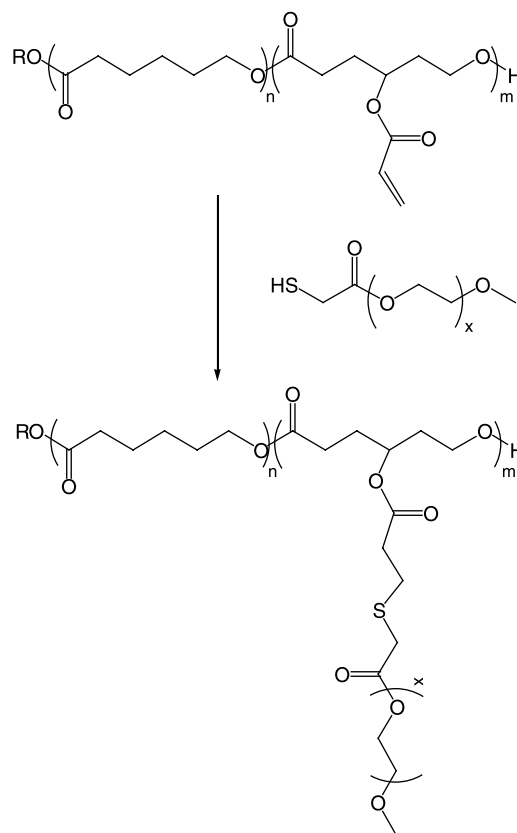
Fig. 41. Graft copolymerization via grafting of thiol terminated PEG to pendant acryloxy side groups on a poly( \epsilon -caprolactone) derivative.
