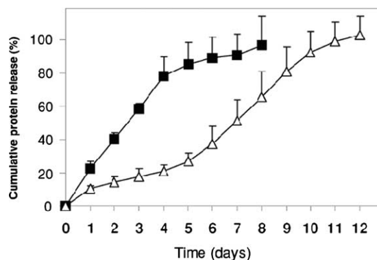
Fig. 48. Release of albumin from PEG networks based on PEG tetraacrylate (black squares) and PEG octaacrylate (white triangles). The lower functionality of the PEG tetraacrylate leads to lower crosslink density and more rapid release. Reprinted from J. Control Rel, 76, Hubbell et al. 'Protein delivery from materials formed by self-selective conjugate addition reactions,' 11–25, Copyright 2001, with permission from Elsevier [9].
