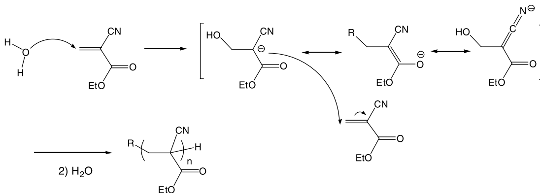
Fig. 30. Water-initiated polymerization of ethyl \alpha -cyanoacrylate.
