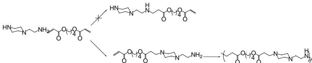
Fig. 38. Hyperbranched poly(ester amine)s from A_2 + B_3 polymerization with unequal reactivity in the B_3 monomer functional groups.
