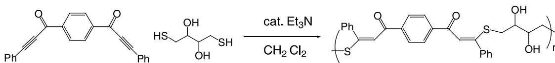
Fig. 24. Poly(enone sulfide) synthesis via Michael addition step growth.
