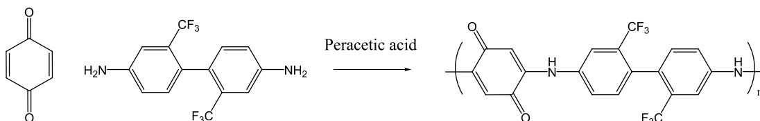
Fig. 22. Poly(amino quinone) synthesis involving peracetic acid as an oxidizing agent.
