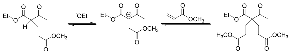
Fig. 3. Second Michael addition of acetoacetate group to methyl acrylate.
