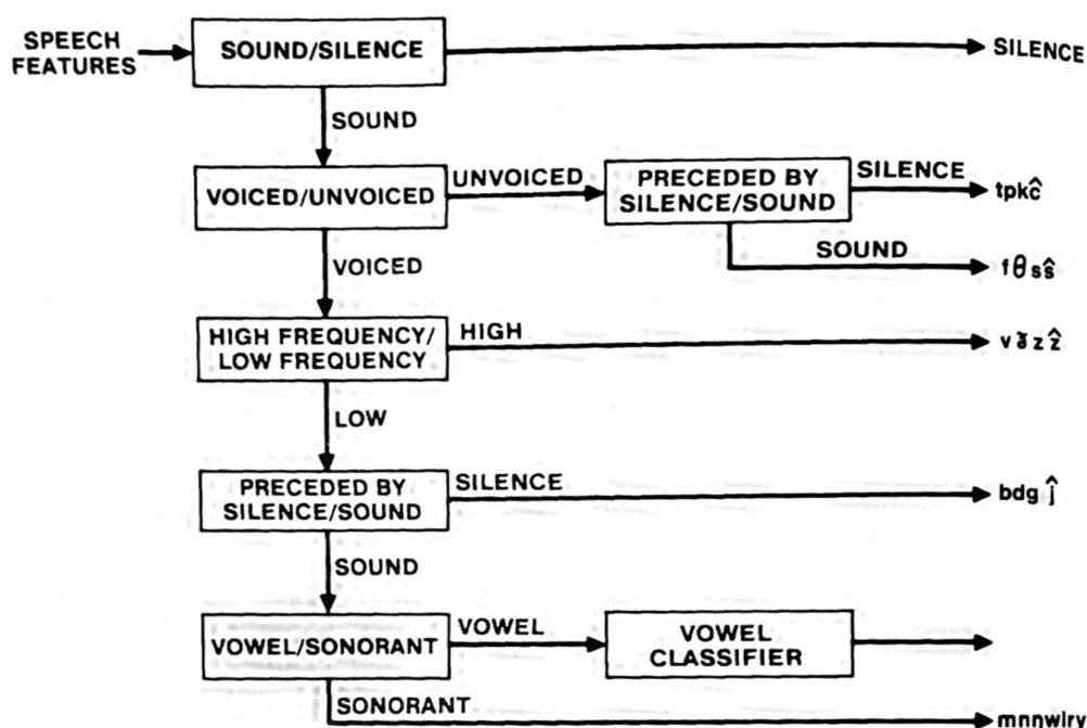
Figure 2.34 Binary tree speech sound classifier.
