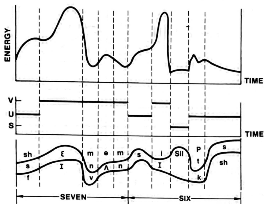
Figure 2.35 Segmentation and labeling for word sequence "seven-six."
