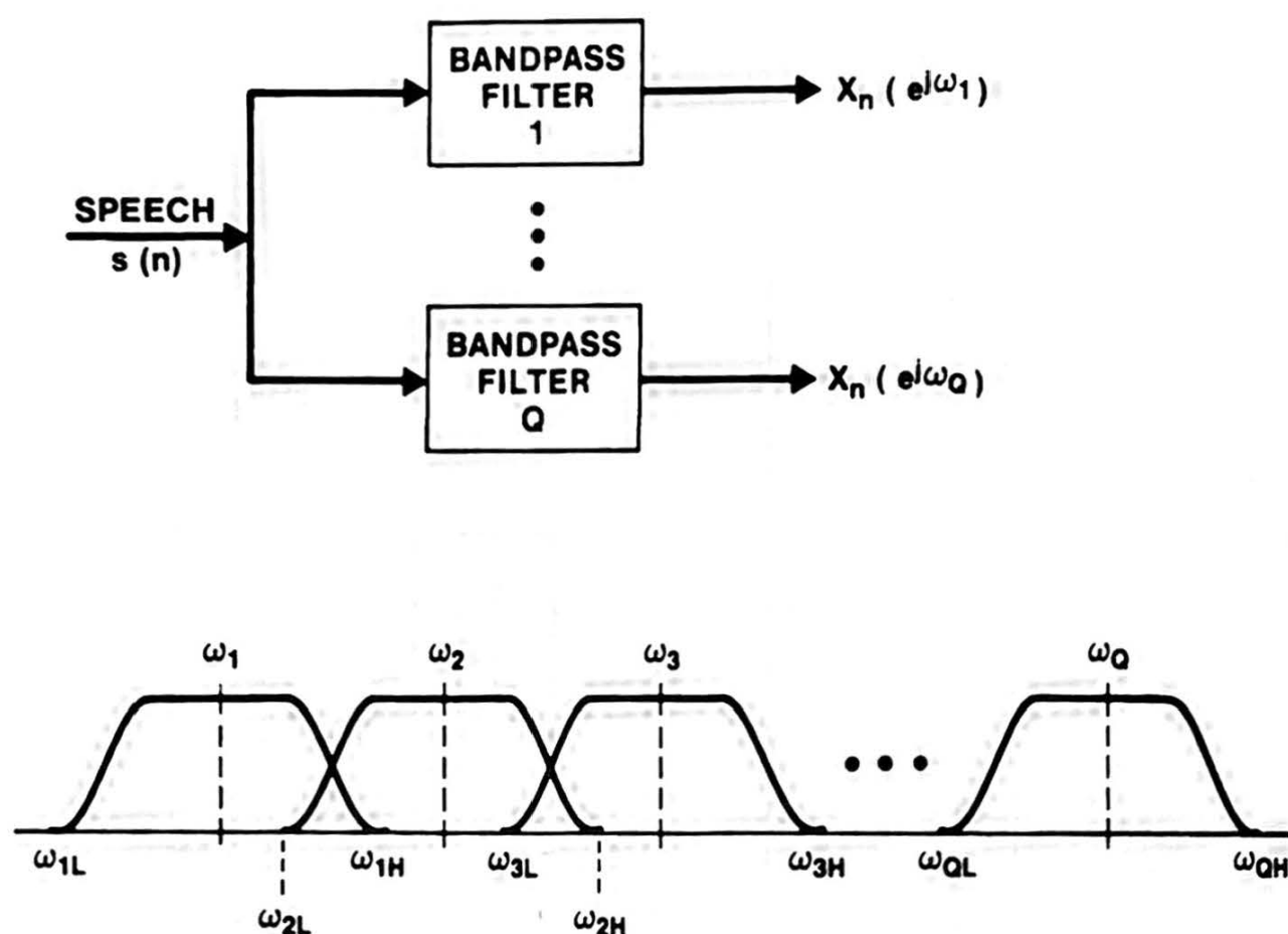
Figure 3.2 Bank-of-filters analysis model.
