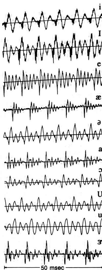
Figure 2.14 Acoustic waveform plots of typical vowel sounds.
