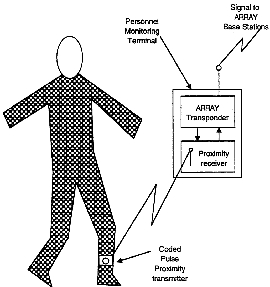
Block Diagram of Personnel Monitoring System
