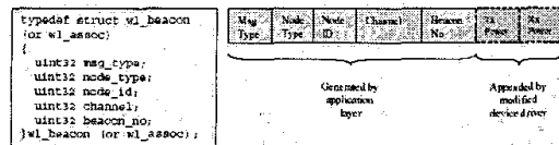
Figure 4. Beacon and Association Message Format
