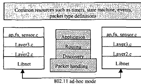
Figure 5. Software architecture of SOHAN
