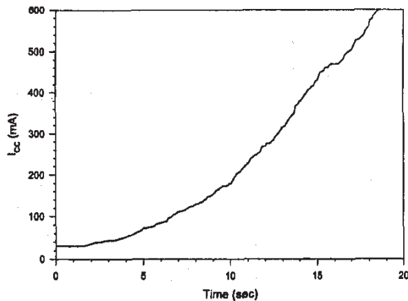
Figure 10. I_{CC} of a non-programmed B4 part during Br ion ( LET = 37 \text{ MeV-cm}^2/\text{mg} ) bombardment.
