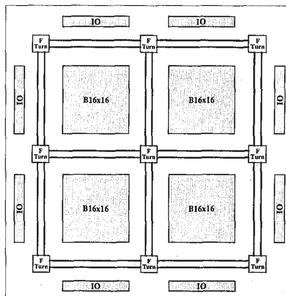
Figure 2. Floor plan of a four B16x16 tile (B4) RS device
