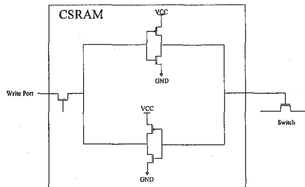
Figure 1. The schematics of the CSRAM controlled switch.
