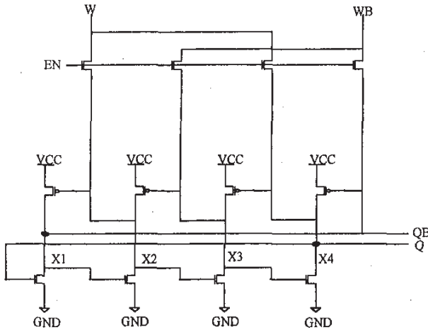
Figure 9. Schematic of the DICE SRAM.
