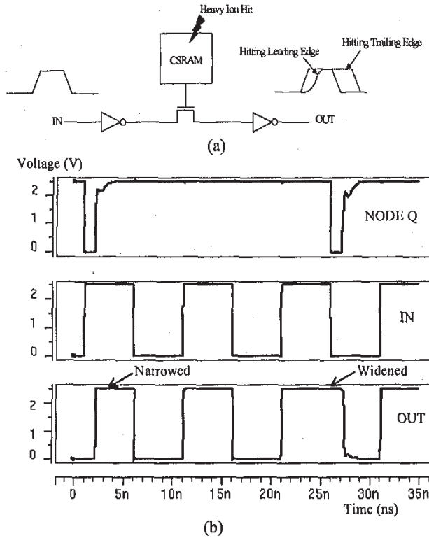
Figure 6 Mode 2 single event transient, metastability in CSRAM modifies the data signal.
