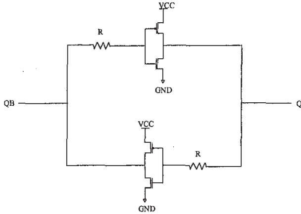
Figure 8. Resistor hardened SRAM.
