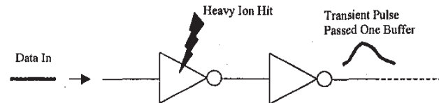
Figure 5. Mode 1 single event transient in combinational logic.
