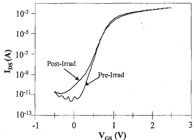
Figure 11. I_{DS} - V_{GS} of a 0.25 \mu\text{m} NMOSFET pre- and post-100krad(Si) irradiation
