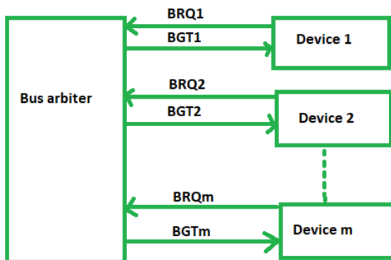
Fixed priority bus arbitration method
