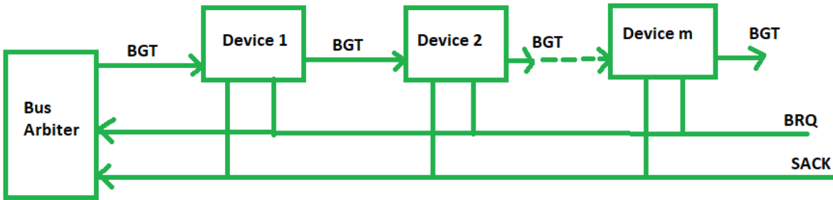
Daisy chained bus arbitration
