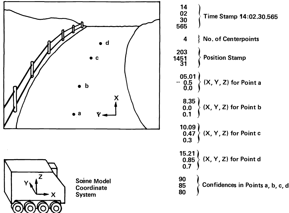
Figure 8. Road scene and corresponding scene model.
