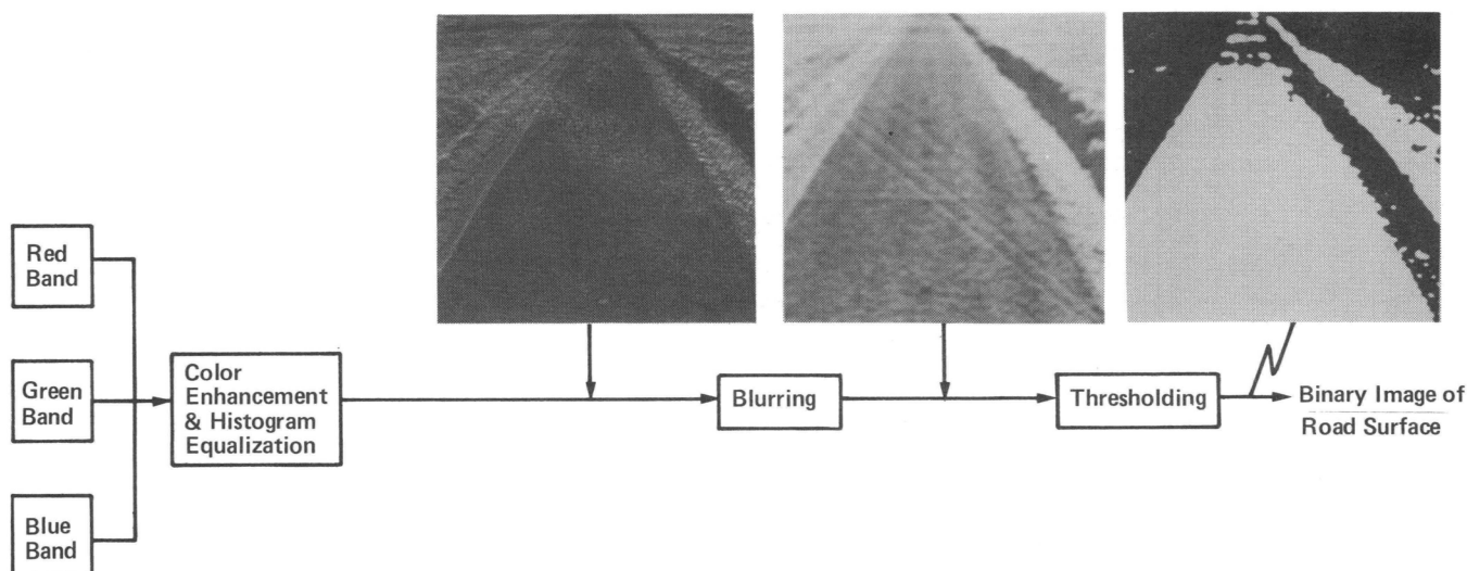
Figure 10. Road segmentation.
