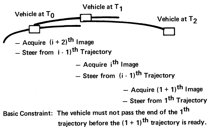
Figure 6. Reference trajectory concept.
