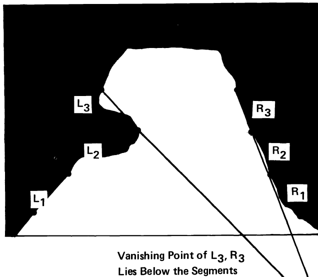
Figure 13. Road with diverging edges.
