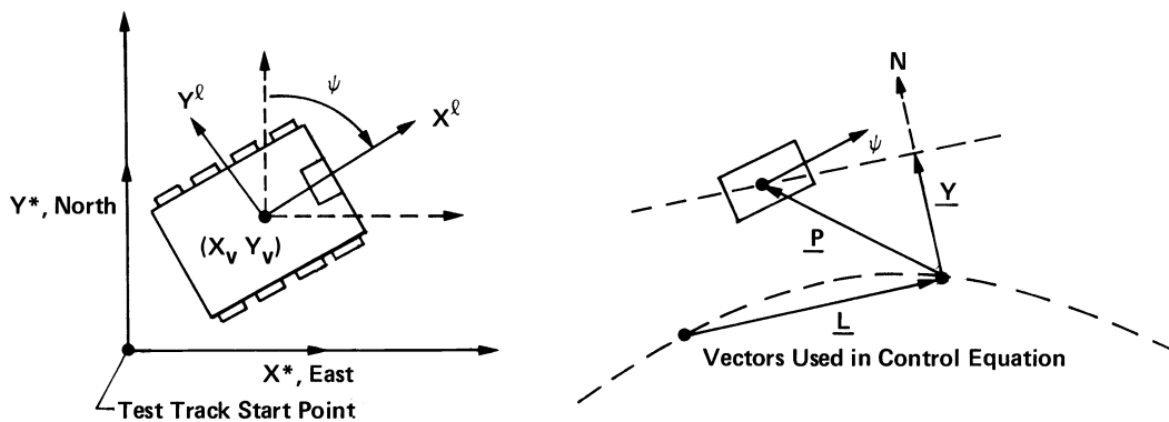
Figure 15. Fixed and local (vehicle) coordinate systems.
