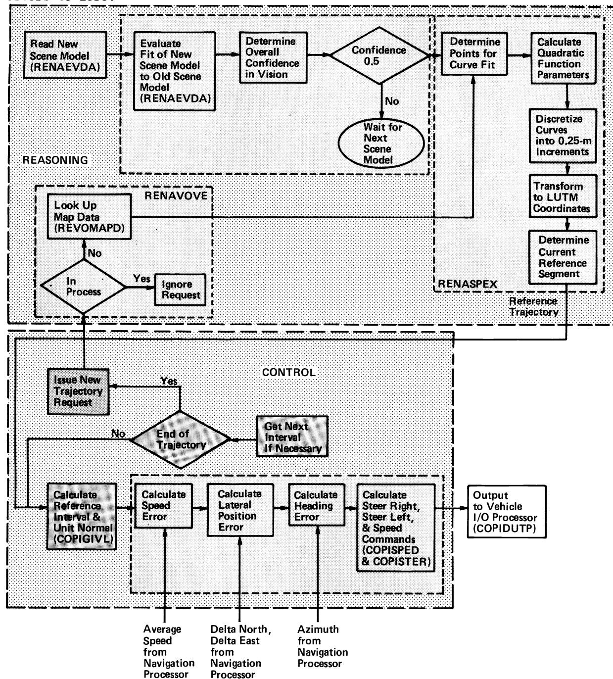
Figure 14. Reasoning and control components.
