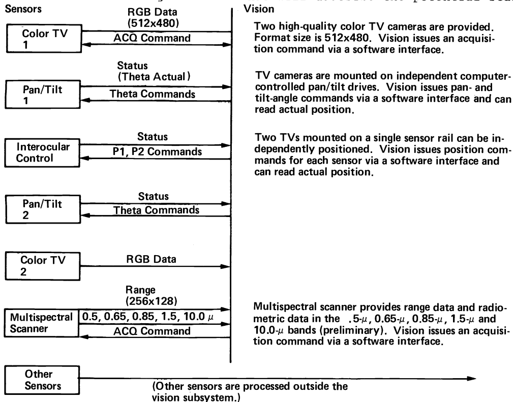
Figure 2 Sensor/Perception Interface
