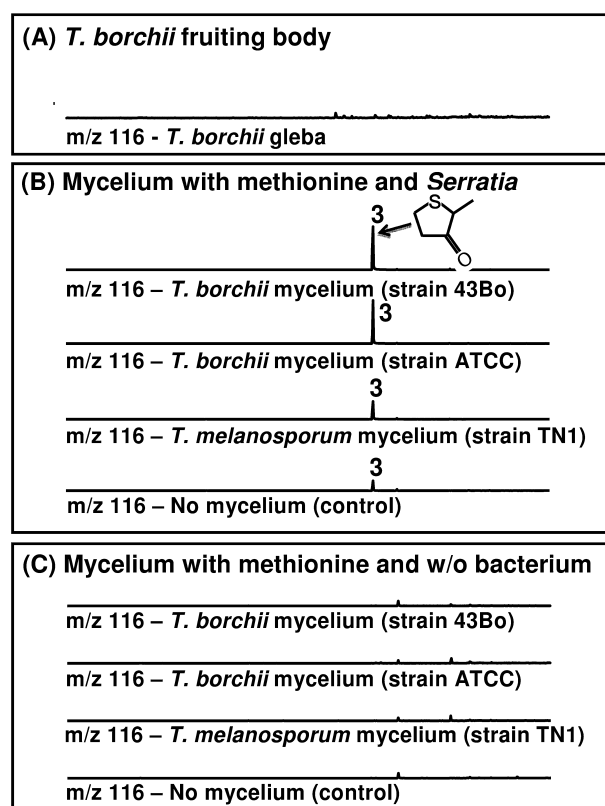
Fig. 5. Methionine induces thiophene derivative 2-methyltetrahydrothiophen-3-one in Serratia . A. Volatile (3) was not detected from T. borchii fruiting bodies. B. It was detected whenever the bacterium was present. C. It was not detected when the bacterium was absent. Chromatograms (extracted mass m/z 116) are shown with normalized intensities.
