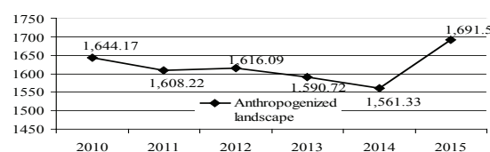
Figure 2. Anthropogenized landscape change of Kaunas city in hectares during the period between the years 2010 and 2015.
