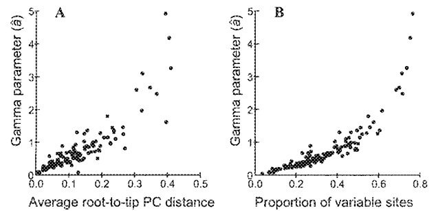
Fig. 2. (A) Relationship between estimated gamma parameter ( \hat{a} ) and the average root-to-tip distance ( b_R ) for 104 nuclear proteins from the five species used. (B) Relationships between \hat{a} and the proportion of variable sites ( p_v ) among the five sequences.
