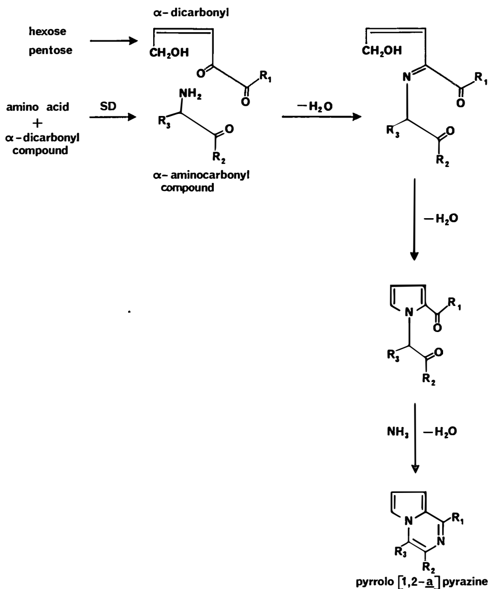
FIGURE 7. Formation of pyrrolo [1,2-a] pyrazines. (From Flament, I., et al., Helv. Chim. Acta , 60, 1877, 1977. With permission.)
