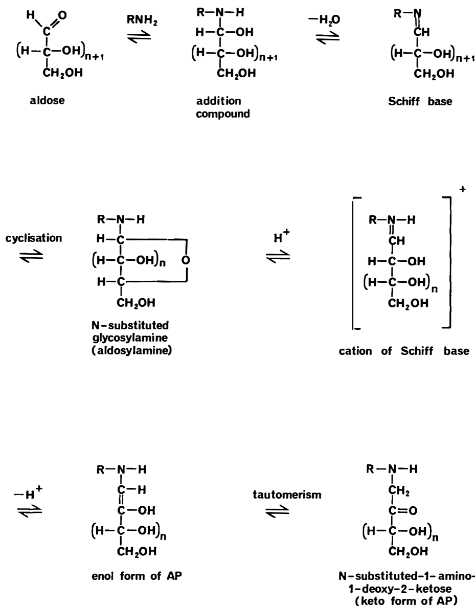
FIGURE 2. Formation of Amadori product (AP) from aldose + amine. (Adapted with permission from Hodge, J. E., J. Agric. Food Chem. , 1, 931, 1953. American Chemical Society.)
