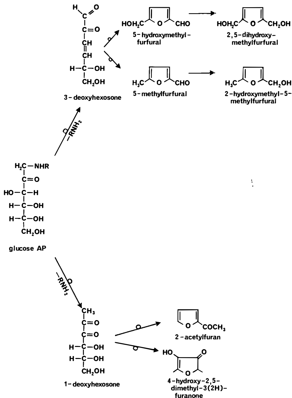
FIGURE 4. Formation of furanoid compounds from glucose Amadori compound. 102 (From Tressl, R., et al., Progress in Flavor Research , Applied Science, London, 1979, 198. With permission.)
