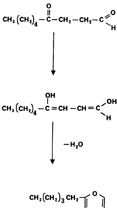
FIGURE 12. Proposed formation of 2-pentylfuran from 4-ketononanal. (From Chang, S. S., et al., Chem. Ind. , 1927, 1966. With permission.)
