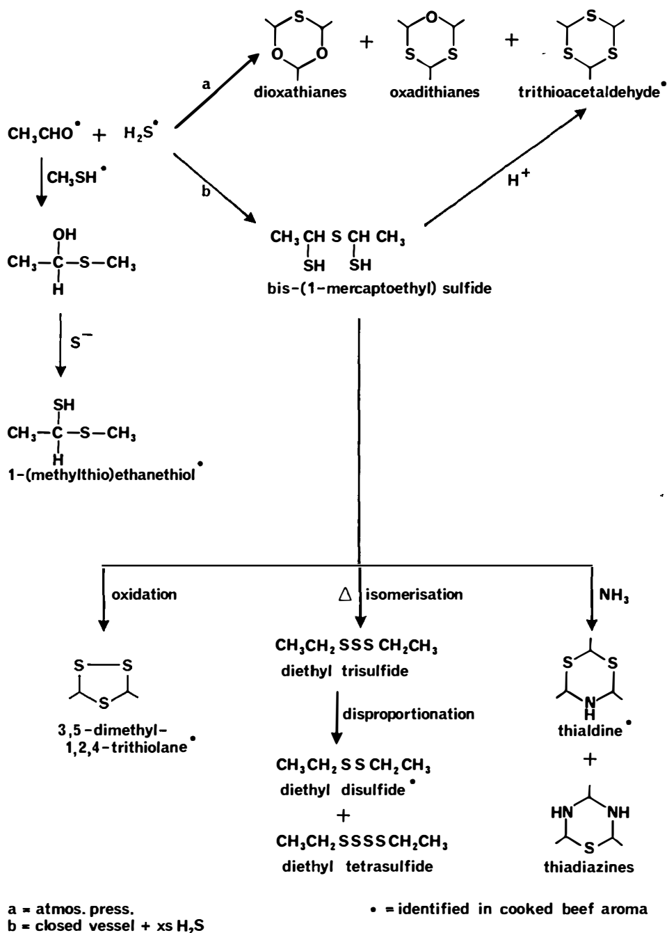
FIGURE 9. Some reactions of aldehydes and hydrogen sulfide. (Reprinted with permission from Takken, H. J., et al., in Phenolic, Sulfur and Nitrogen Compounds in Food Flavors , ACS Symp. Ser. 26, 1976, 116. American Chemical Society.)
