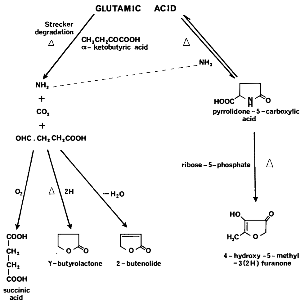
FIGURE 16. Some possible reactions of glutamic acid and \alpha -ketobutyric acid. 3
