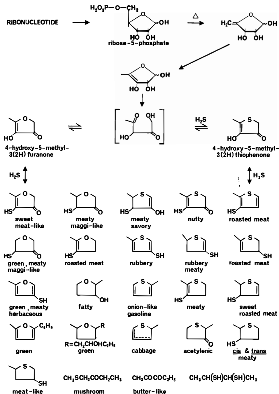
FIGURE 8. Formation from ribonucleotides of 4-hydroxy-5-methyl-3(2H) furanone and its reaction with hydrogen sulfide. 1,98
