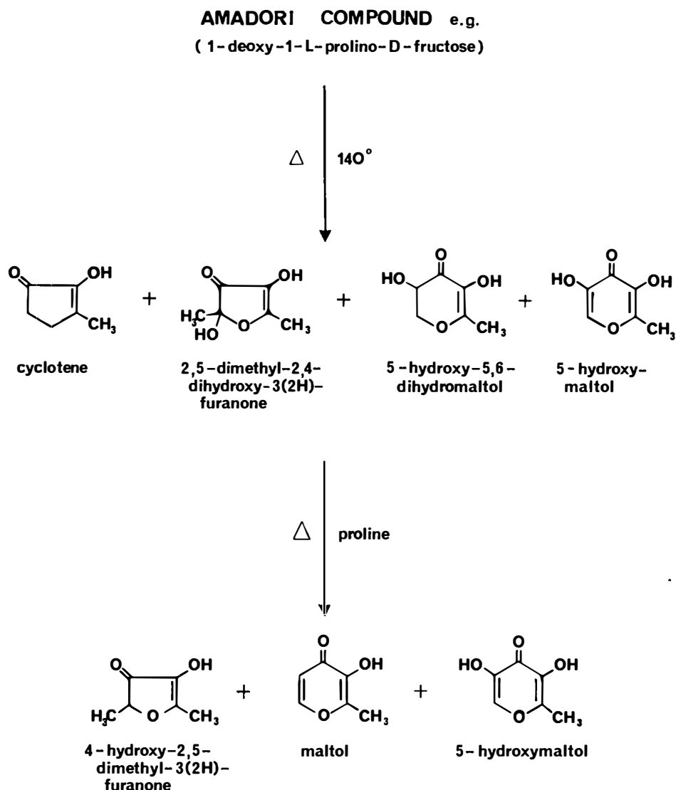
FIGURE 5. Compounds with caramel odors which arise by Maillard reaction. 102,177
