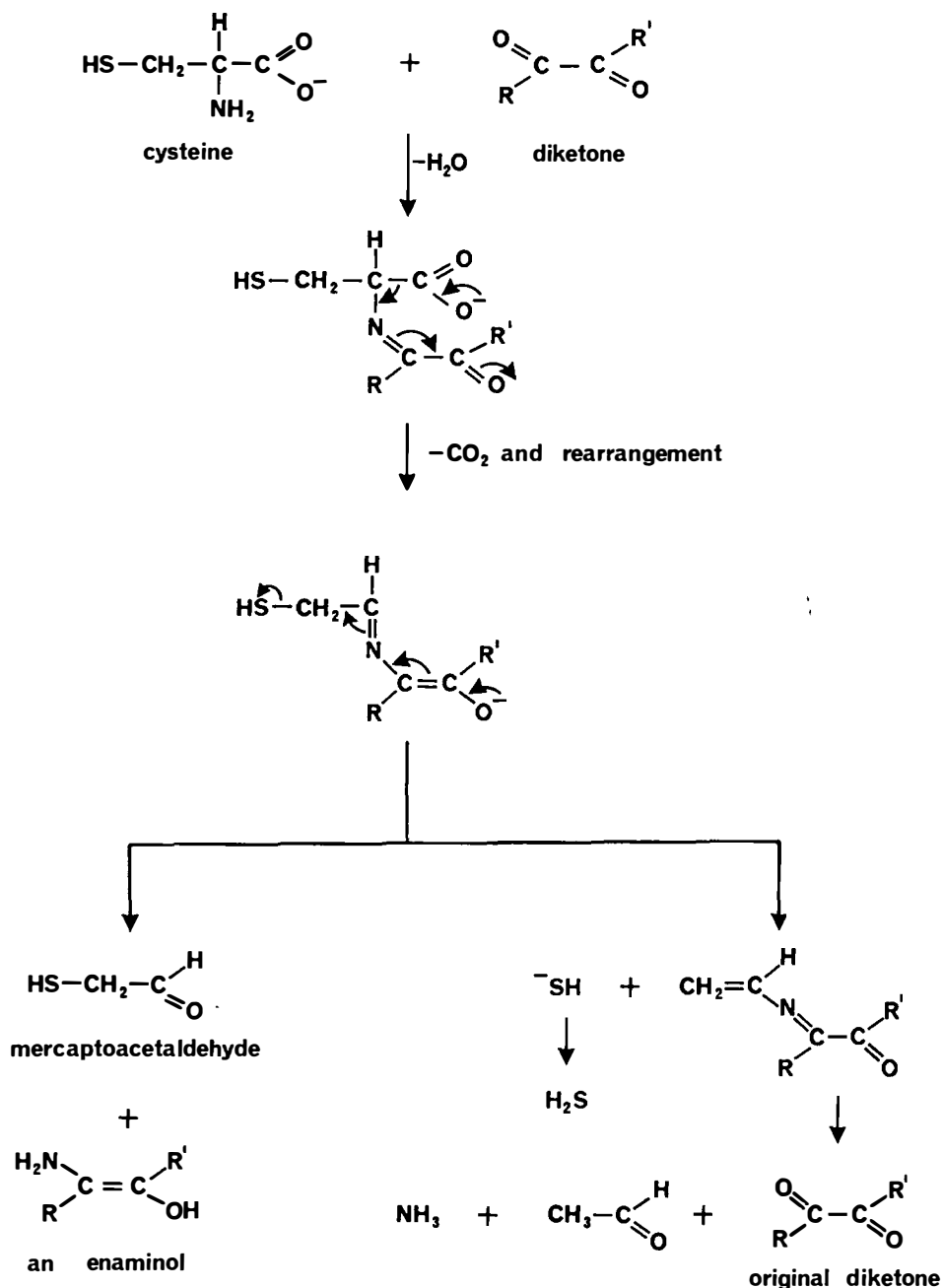
FIGURE 1. The Strecker degradation of cysteine. 1
