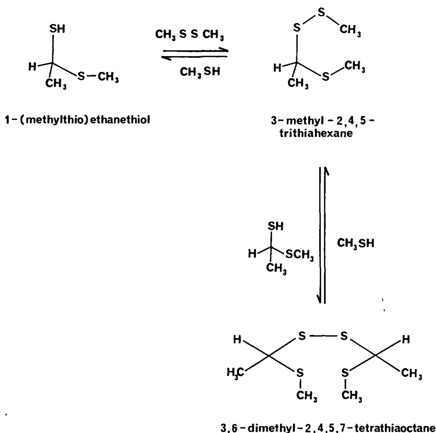
FIGURE 11. Proposed formation of trithiahexanes and tetrathiaoctanes from 1-(methylthio)ethanethiol. (From Dubs, P. and Stüssi, R., Helv. Chim. Acta , 161, 2355, 1978. With permission.)
