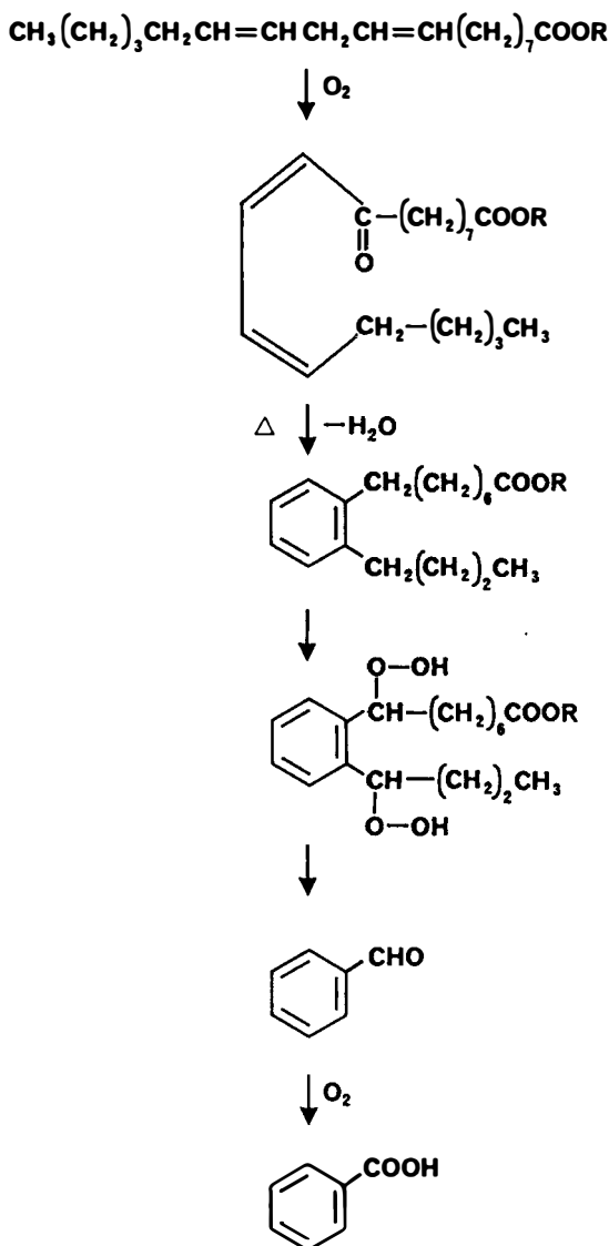
FIGURE 13. Proposed formation of benzoic acid and benzaldehyde from linoleate. (From Kawada, T., et al., J. Am. Oil. Chem. Soc. , 44, 134, 1967. With permission.)
