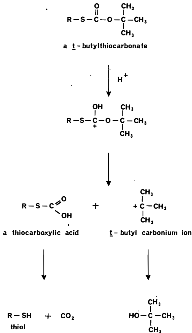
FIGURE 17. Release of thiols from t -butylthiocarbonates. (Reprinted with permission from Schutte, L., in Phenolic, Sulfur and Nitrogen Compounds in Food Flavors , ACS Symp. Ser. 26, 1976, 108. American Chemical Society.)
