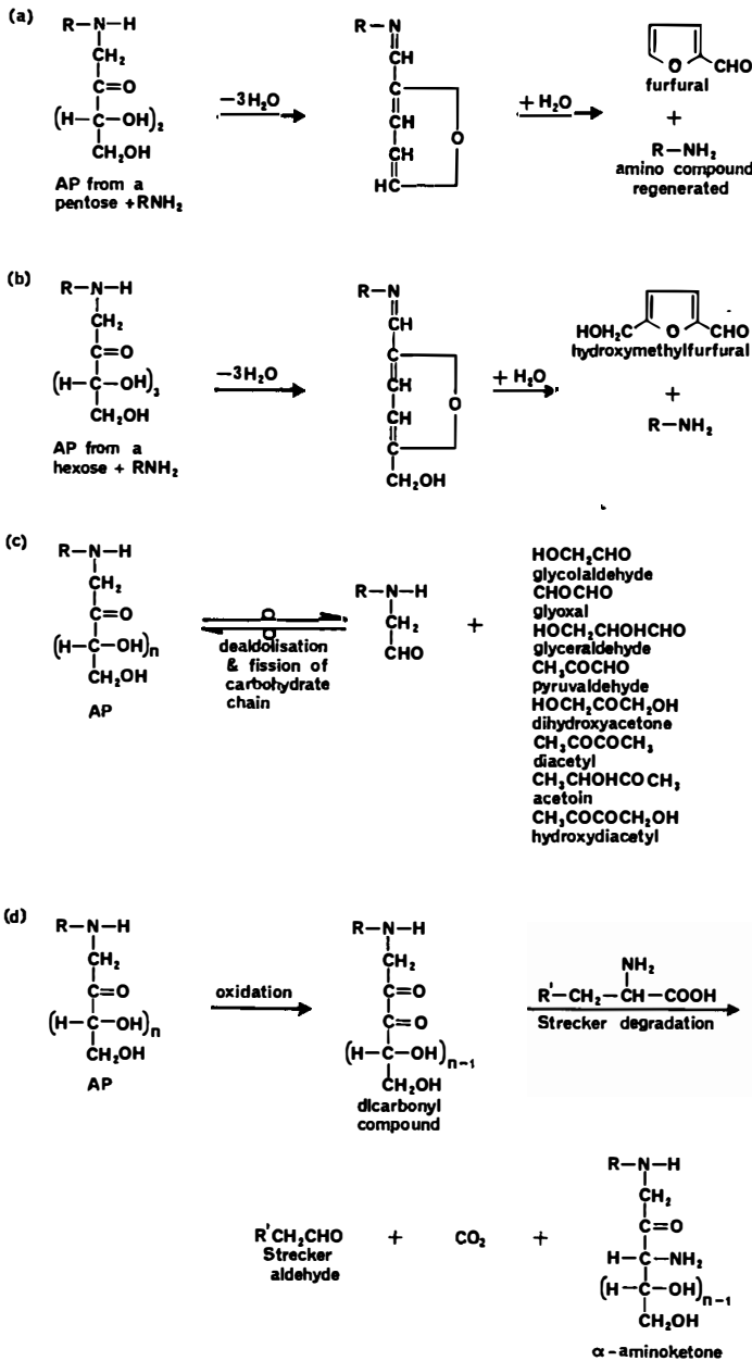
FIGURE 3. Some reactions of Amadori products (APs). 162, 167
