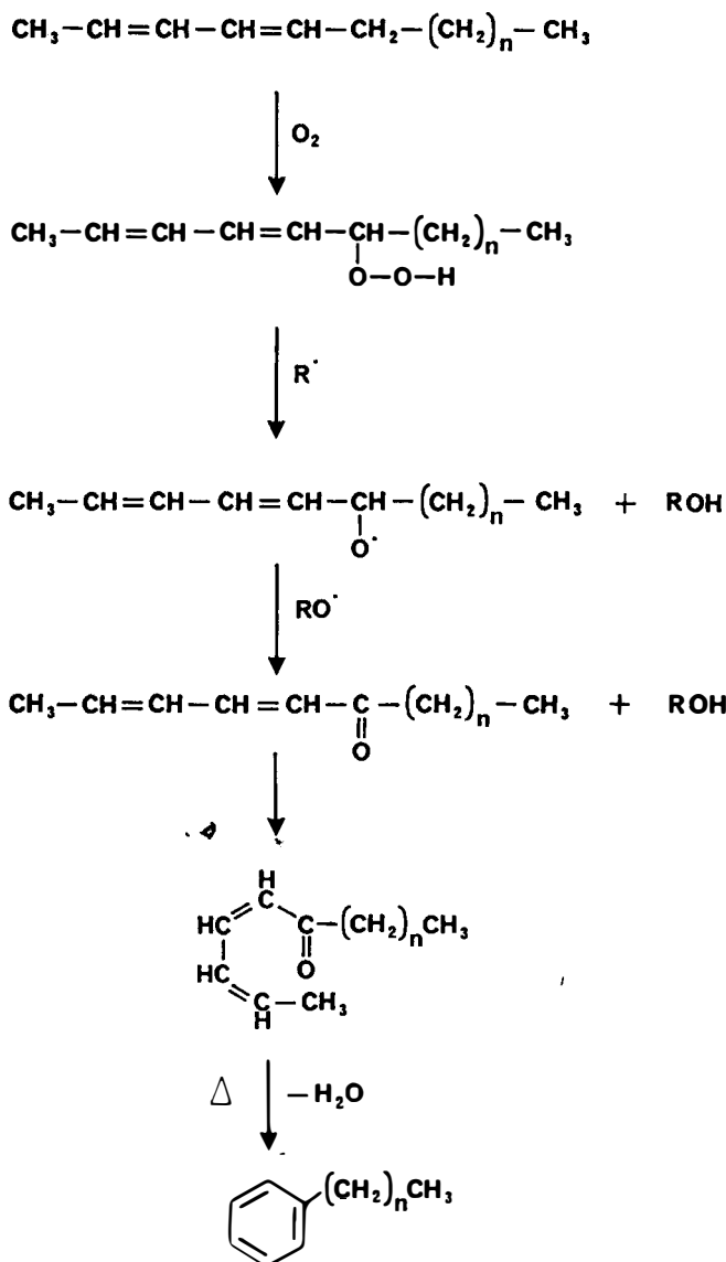
FIGURE 14. Formation of alkylbenzenes from long chain hydrocarbons derived by thermal oxidation of fatty acids. (Reprinted from Min, B. S. D., et al., J. Food Sci. , 42, 504, 1977. Copyright by Institute of Food Technologists.)
