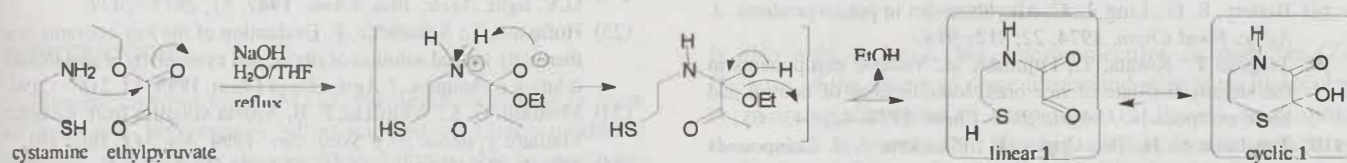
Figure 5. Chemical correlation of N -(2-sulfanylethyl)-2-oxopropanamide by direct synthesis.
