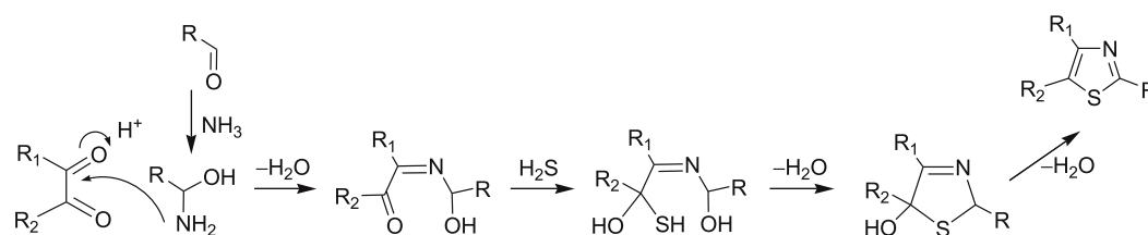
Scheme 12.7 Route for the formation of thiazoles
