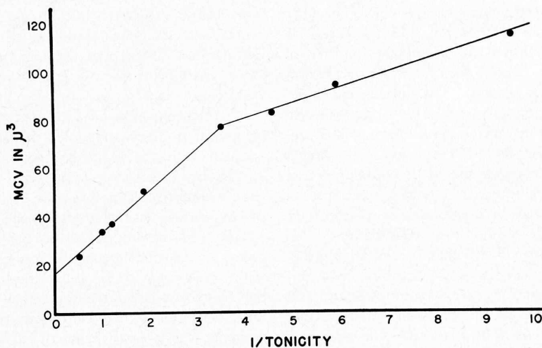
FIG. 1. OSMOTIC RESPONSIVENESS OF HUMAN ERYTHROCYTE GHOSTS CELLS. Mean corpuscular volume of ghosts after addition of buffered sodium chloride is plotted against final extracellular tonicity. 310 mOsm per L was taken as 1.
