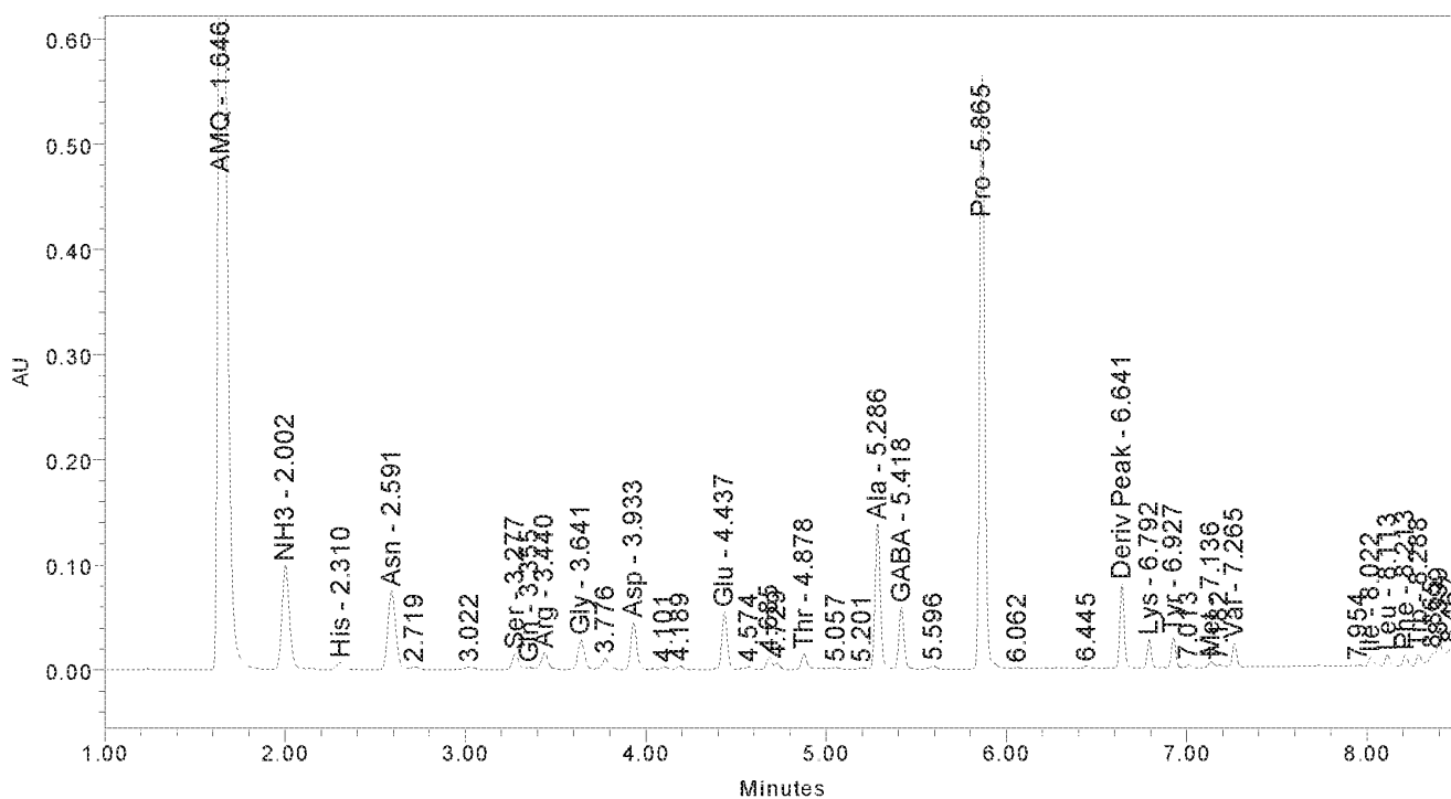
Auto-Scaled Chromatogram
