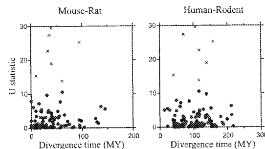
Fig. 3. Relationships between estimated divergence times and U statistic values for each of 104 proteins. The molecular clock hypothesis was rejected for the proteins indicated with the \times symbol.
