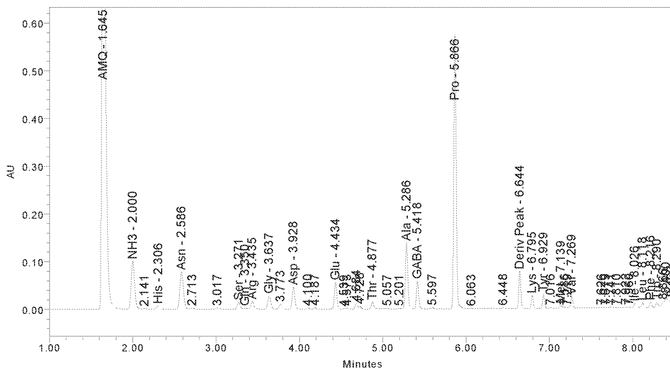
Auto-Scaled Chromatogram
