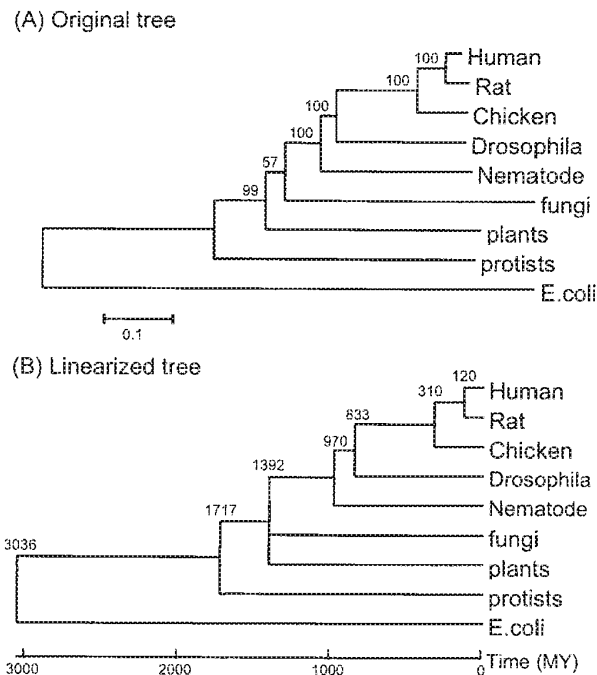
Fig. 4. (A) NJ tree constructed by using distance d_3 with a = 1.24 for 11 protein sequences. The numbers given for this tree stand for the bootstrap values (500 replications). (B) Linearized tree of the above NJ tree. The numbers given for this tree represent the estimates of divergent times.
