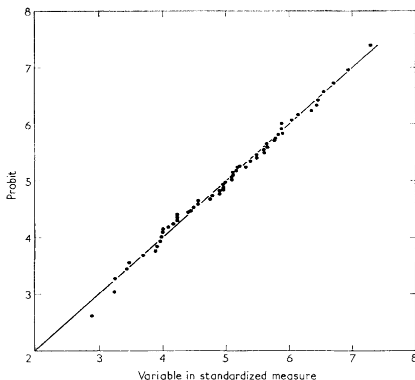
FIG. 3. Probit plot for six grouped random samples.
