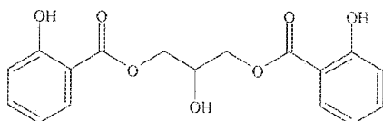
Glycerol Di-Salicylate
