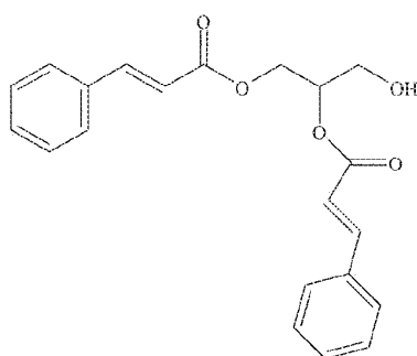
Glyceryl Di-Cinnamate
