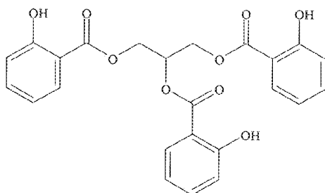
Glycerol Tri-Salicylate
