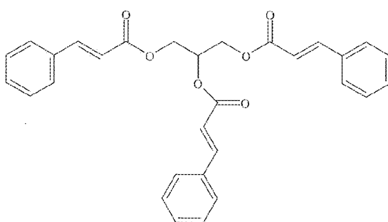
Glyceryl Tri-Cinnamate
