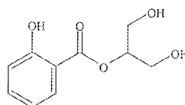
Glycerol Mono-Salicylate
