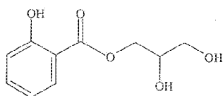
Glycerol Mono-Salicylate
