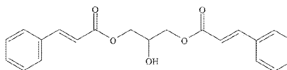
Glyceryl Di-Cinnamate
