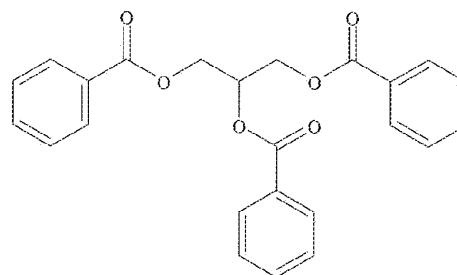
Glyceryl Tri-Benzoate
