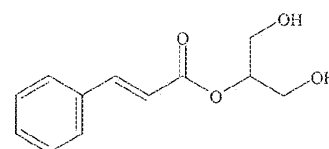
Glyceryl Mono-Cinnamate
