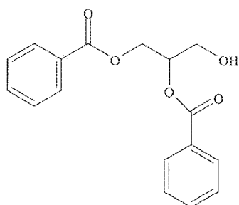
Glyceryl Di-Benzoate
