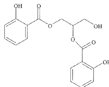
Glycerol Di-Salicylate
