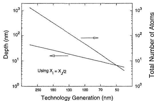
Fig. 5-10 Typical thickness of lighter-doped layer and total number of impurity atoms for 10^{17}/\text{cm}^3 surface doping density. 11
