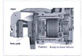
Electric brake Source: Delphi (IEEE IAS Mag, 2009)
