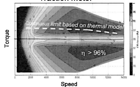
Traction motor
