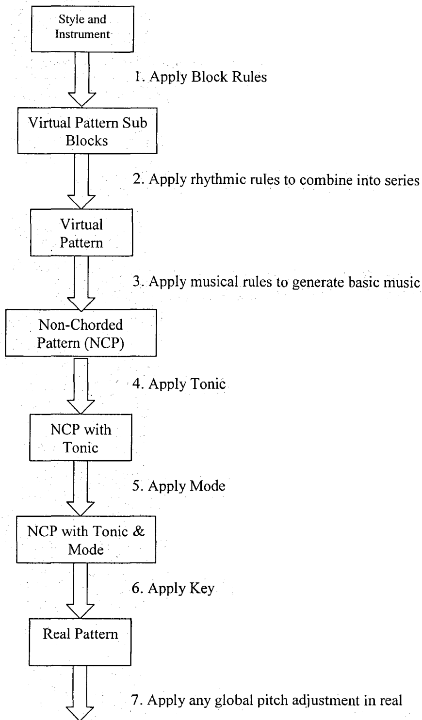
General Musical Generation Flow
