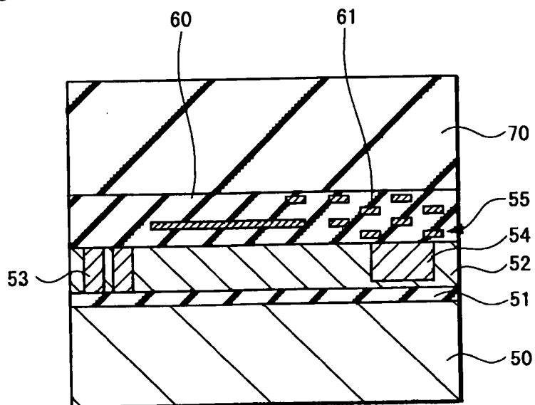
FIG. 4C (RELATED ART)
