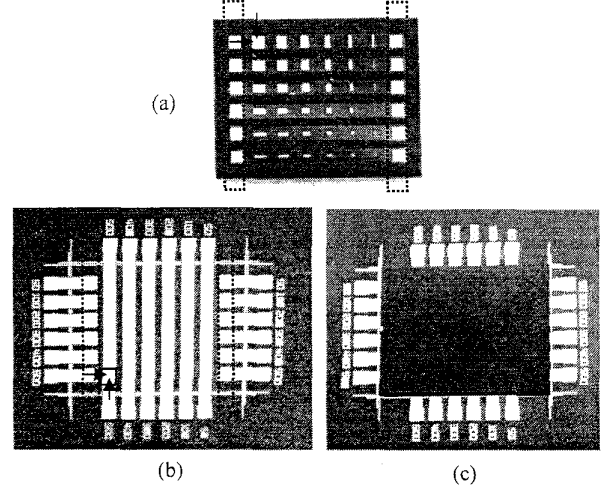
Fig. 6. Microphotographs of flip-chip assembly: (a) flip-chip; (b) substrate; and (c) their assembly used for the contact resistance measurement of the bumps.
