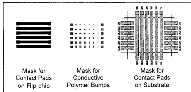
Fig. 4. Three-mask set of test structures to evaluate the electrical properties of the thermoplastic conductive polymer bumps by using a four-point terminal method.
