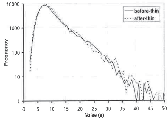
Figure 8: Measured noise histogram
