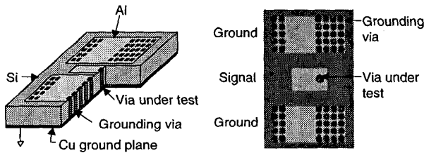
Fig. 6. Left: 3-D schematic of the test structure. The multiple grounding vias are introduced to reduce the impedance of the ground pads. Right: picture of the one-port test structure for measuring the impedance of a single via.
