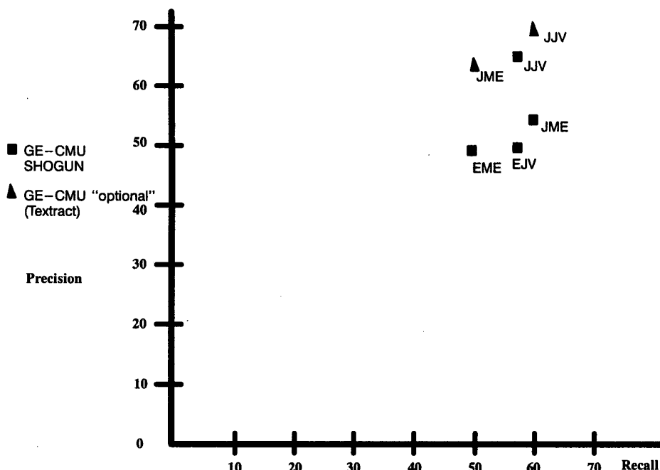
Figure 3: GE-CMU Results for MUC-5/TIPSTER 24-month benchmark
