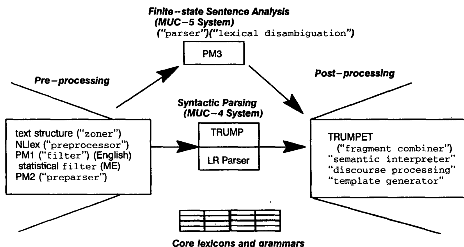
Figure 1: SHOGUN configuration in MUC-5
