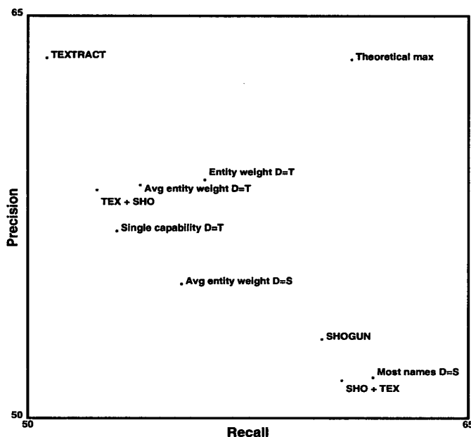
Figure 6: Combining Two MUC-5 Systems: Graph
