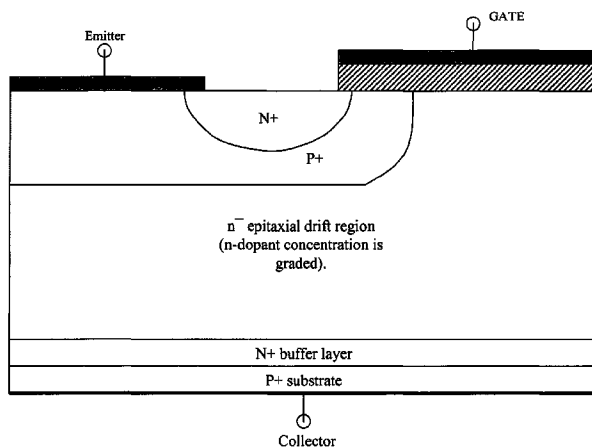
A dopant - concentration graded drift region in a IGBT
