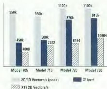
Fig. 9. Graphics performance comparison.
