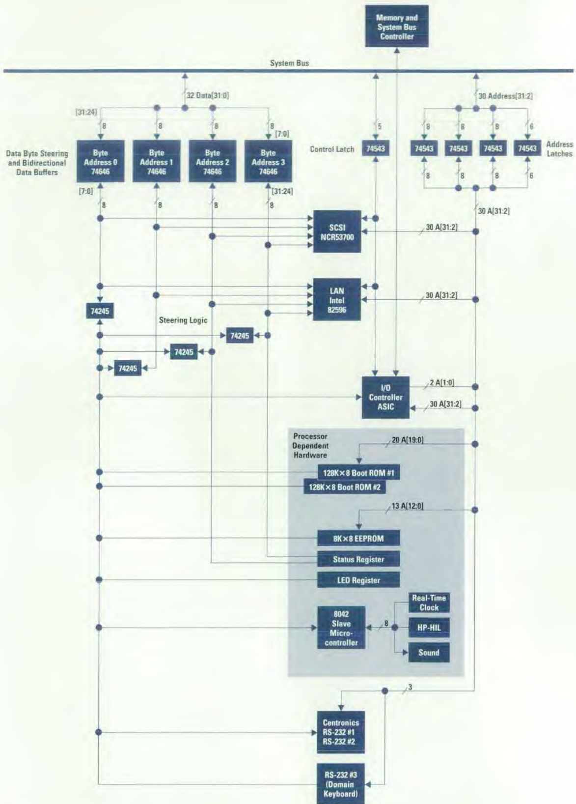
Fig. 1. HP 9000 Series 700 I/O subsystem block diagram.
