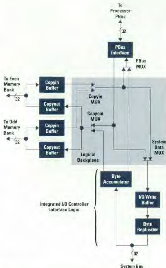
Fig. 4. Memory and system bus interface data path.
