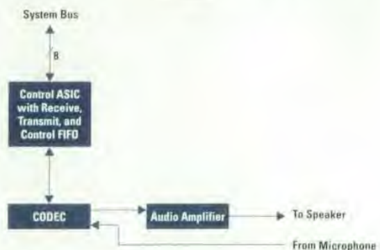
Fig. 7. Audio CODEC (coder/decoder) and FIFO buffer diagram.
