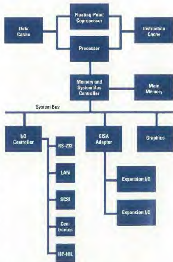
Fig. 1. HP 9000 Series 700 system block diagram.
