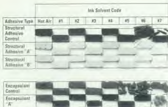
Fig. 1. Adhesive test blocks after accelerated stress tests.
