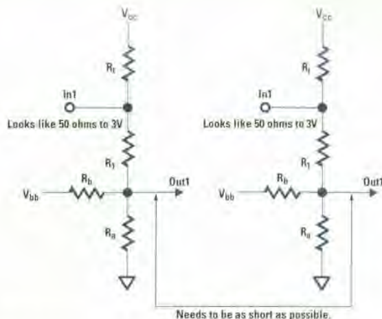
Fig. 2. Passive differential level translation circuit.
