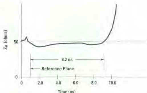
Fig. 4. TDR measurement of an unterminated 4.4-ns clock system delay line.
