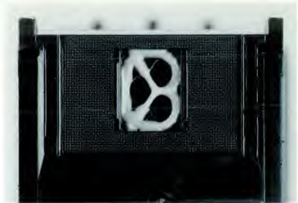
Fig. 2. Adhesive pattern dispensed by the production equipment
