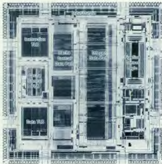
Fig. 4. CPU chip.
