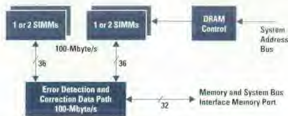
Fig. 5. Memory bank controller
