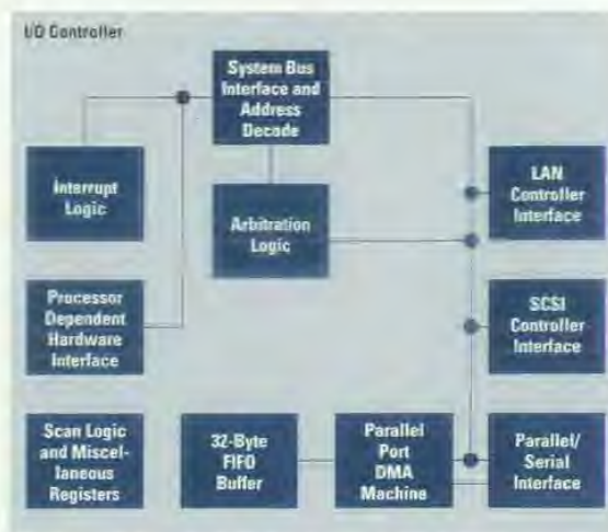
Fig. 2. I/O controller ASIC chip block diagram.
