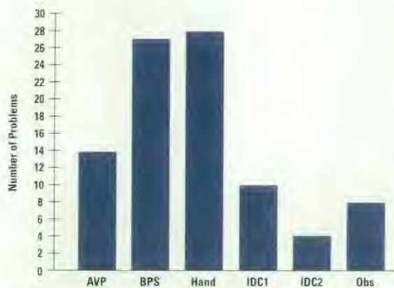
Fig. 1. Number of bugs found by each test class.
