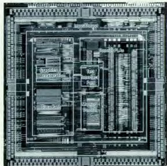
Fig. 7. Memory and system bus controller chip.
