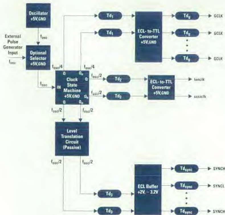
Fig. 1. HP 9000 Series 700 workstation clock system block diagram. All active clock components are on the CPU board except the ECL-to-TTL converter that drives lanch and sasiclk.
