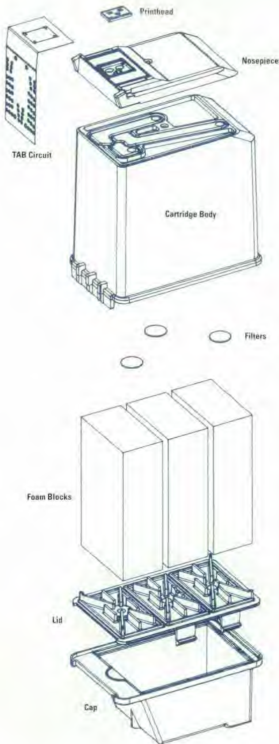
Fig. 1. Exploded view of the color print cartridge.
