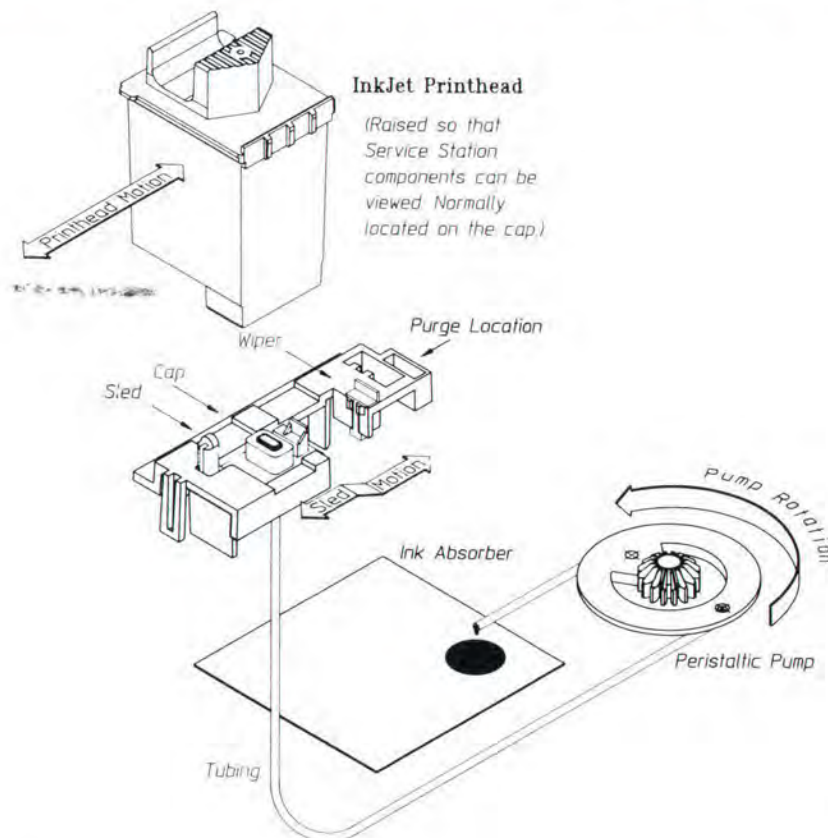
Fig. 3. DeskJet printer service station assembly.
