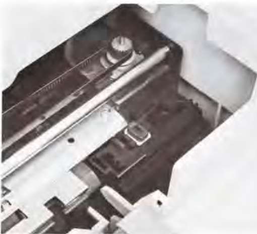
Fig. 4. Photograph of the service station.
