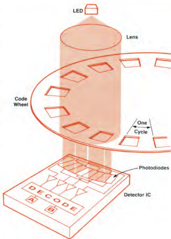
Fig. 2. Optical arrangement of the HEDS-9000 encoder. There are four photodiodes per code wheel cycle (one spoke and window pair). All four contribute to both output channels (A and B).
