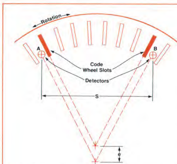
Fig. 2. Lines on a code wheel radically displaced by a distance e no longer overlap targets on the detector. This leads to a change in timing for events seen by the two detectors, A and B. This change in timing is a phase error.
