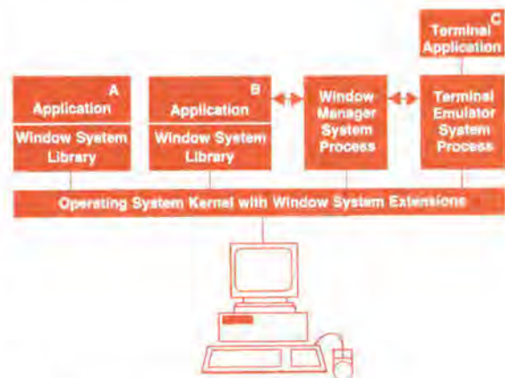
Fig. 1. Conventional window system architecture.
