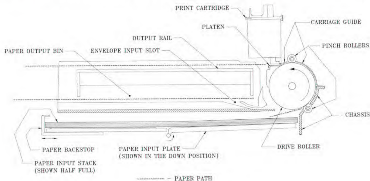
Fig. 2. DeskJet printer paper handling mechanism.
