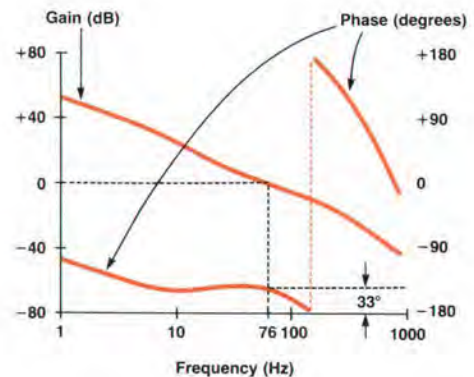
Fig. 7. Loop gain of the high-gain positioning servo. (a) Uncompensated. (b) Compensated.
