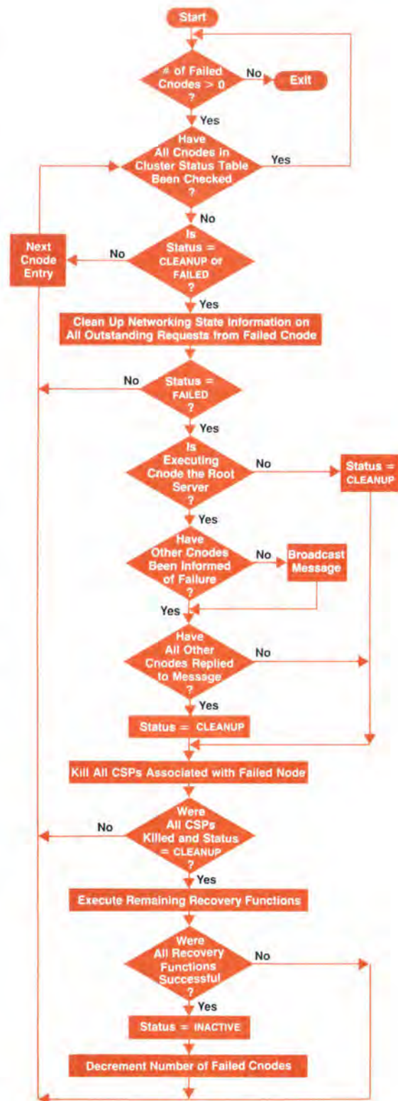
Fig. 4. General crash recovery mechanism (recovery CSP).
