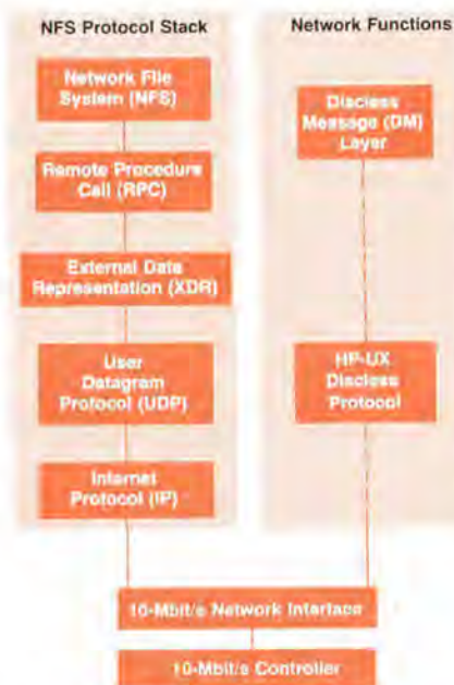
Fig. 2. NFS protocol stack versus HP-UX network functions.
