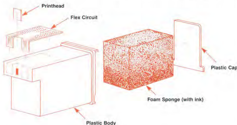
Fig. 9. Exploded view of the DeskJet print cartridge.
