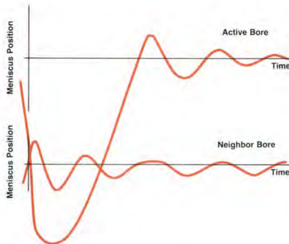
Fig. 4. Fluid damping and cross talk for the initial ink channel length.
