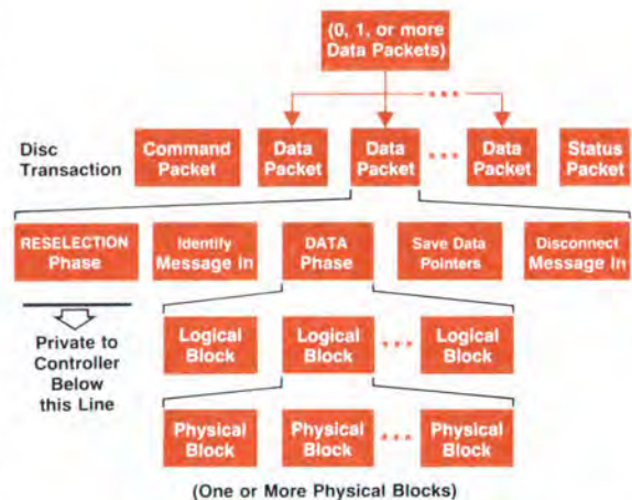
Fig. 3. Data packets for a typical disc transaction on the SCSI bus. The Command packet contains the information for setting up the environment for data transfer. Information such as the Identity and the Synchronous messages are contained in this packet.
