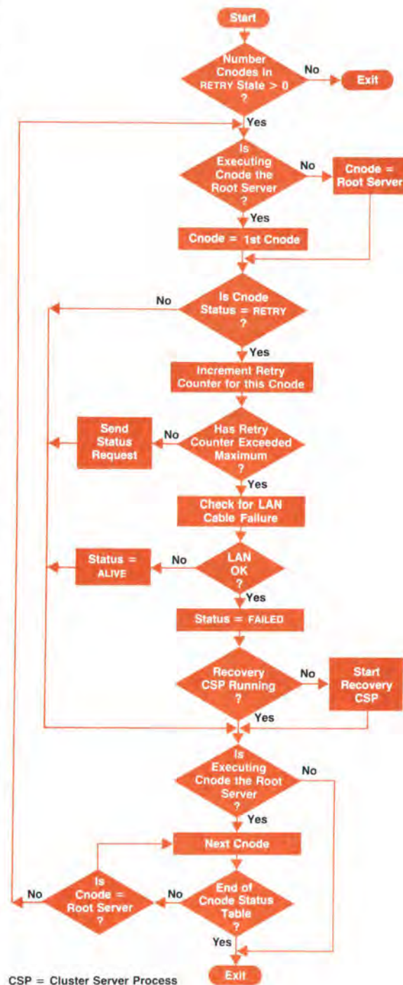
Fig. 3. Crash detection: retry status request process.
