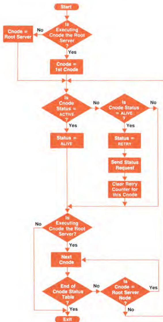
Fig. 2. Crash detection: status checking process.
