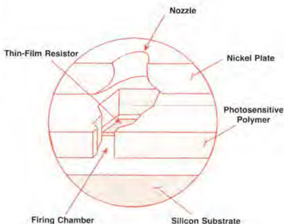
Fig. 2. Cross section of an inkjet nozzle.
