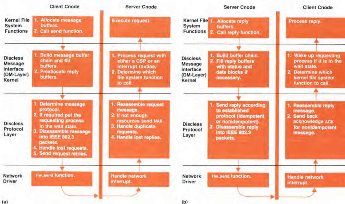
Fig. 3. Network control flow. (a) Originating a request from the client and receiving a request at the server. (b) Sending a reply from the server and receiving a reply at the client. CSP = cluster server process.
