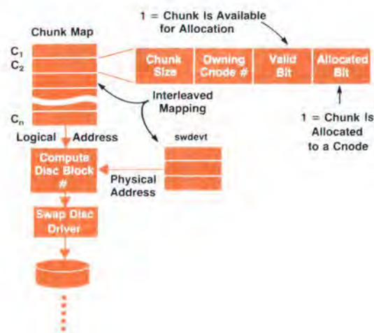
Fig. 4. The chunk map entry.
