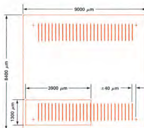
Fig. 2. Overall and single-camera (lower left) fields of view for the TAB prep machine.
