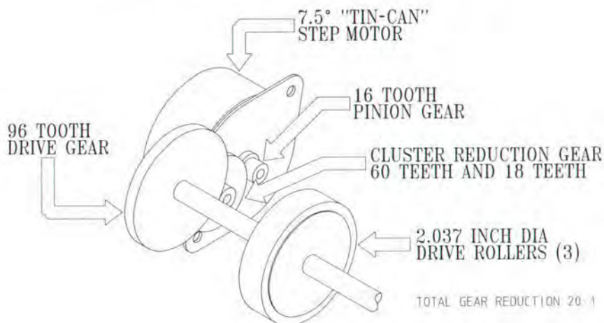
Fig. 4. Paper drive motor assembly.
