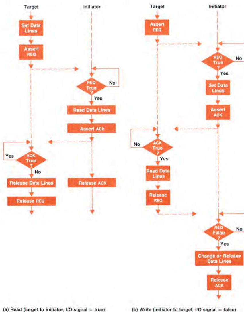
Fig. 2. REQ/ACK handshake protocol.
