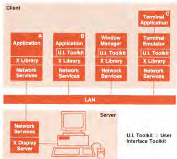
Fig. 2. X Window System client-server architecture.
