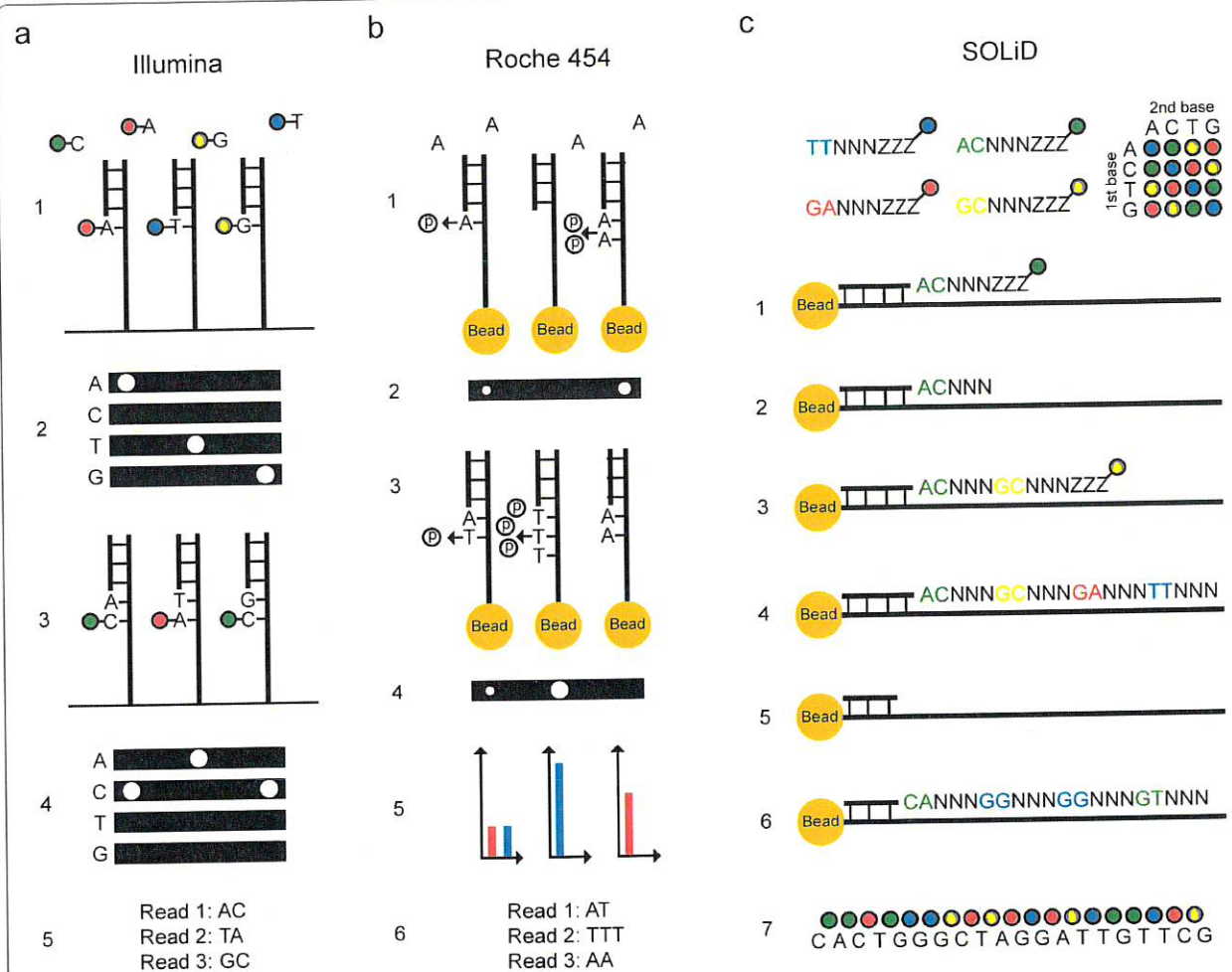
Figure 3 Principles for sequencing and imaging. (a) Illumina sequencing of three template molecules. All four nucleotides, carrying terminating moieties and unique fluorescent labels, and DNA polymerase are added, and one complementary nucleotide becomes incorporated at each template molecule (1). After washing, fluorescence is registered at four wavelengths (2). Fluorescent dyes and terminating groups are cleaved off. A new set of nucleotides is added (3), and imaged (4). Sequence reads of equal length are obtained (5). (b) 454 sequencing of three template molecules. One type of natural non-terminating deoxynucleotides and DNA polymerase are added and a pyrophosphate molecule is released at each nucleotide incorporation (1). Pyrophosphate is converted into light using sulfurylase and luciferase, and the light intensity is measured in each well (2). Free deoxynucleotides are destroyed with apyrase before adding the next type of deoxynucleotide (3) and imaging (4). Light signals are converted to flowgrams with higher signal intensity bars in homopolymer regions (5). Sequence reads that may differ in length are obtained (6). (c) SOLiD sequencing of one template molecule. A sequencing primer, DNA ligase and 1,024 unique probes, which are fluorescently labeled according to their first two bases, are added, and the complementary probe is ligated to the template (1). After washing, fluorescence is registered at four wavelengths. The three universal bases and the fluorophore are cleaved off (2). Addition of a new probe set is repeated for the desired number of cycles (3,4). The newly built strand is melted off. A new sequencing primer is added, which anneals one base off from the first primer and therefore interrogates different positions (5). Sequencing is repeated for the desired number of cycles (6). Additional primers are added, until each base is sequenced twice. The colors from all sequencing rounds are merged and can be converted to nucleotides (7).
