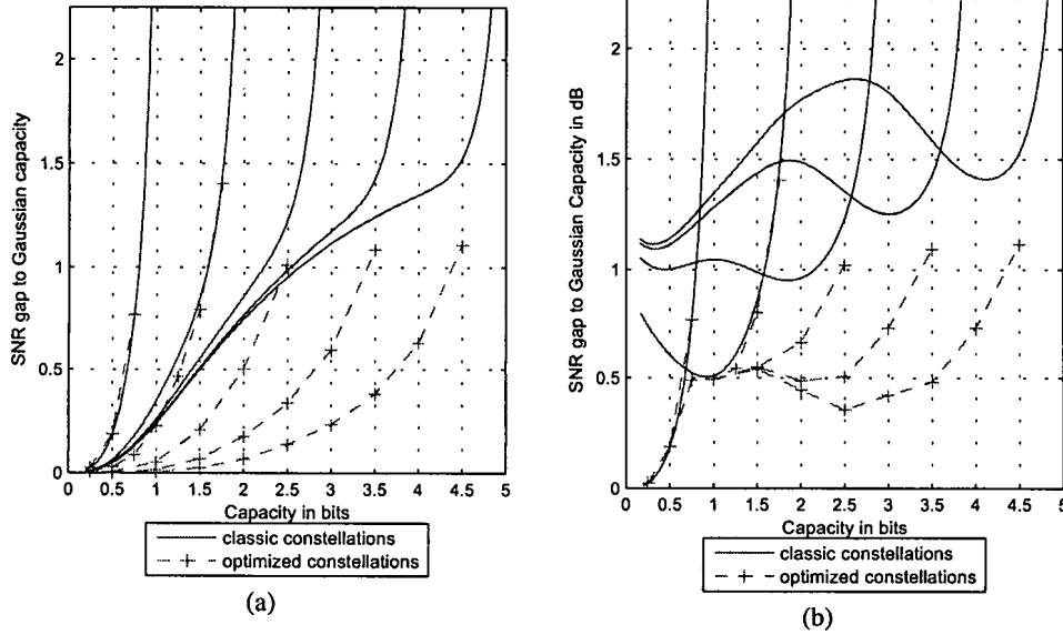
Fig. 4. (a) SNR gap to Gaussian Capacity for the joint capacity of the classic and the optimized PAM 2,4,8,16 and 32 constellations (from left to right respectively). (b) Gap between the Parallel Decoding Capacity and Gaussian Capacity for the optimized and the classic constellations.
