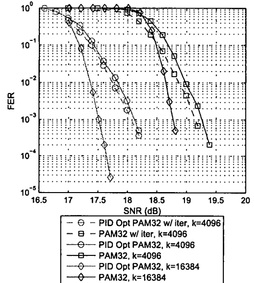
Fig. 6. Simulation results for a BICM system using a rate 1/2 LDPC code for the classic and the optimized PAM 32 constellation
