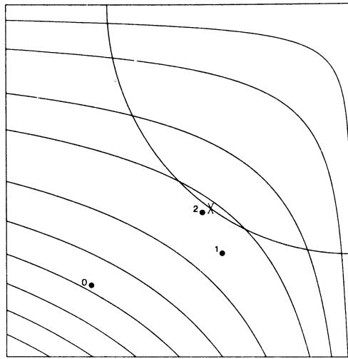
Figure 6I. The first three iterates of a projected Lagrangian method when applied to Example 6.2. Each iterate is the solution of a linearly constrained subproblem.
