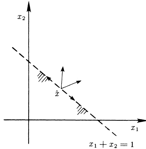
Figure 3h. Feasible directions with respect to the linear constraint x_1 + x_2 \geq 1 .
