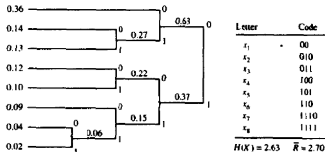
FIGURE 3-3-6 Huffman code for Example 3-3-2.
