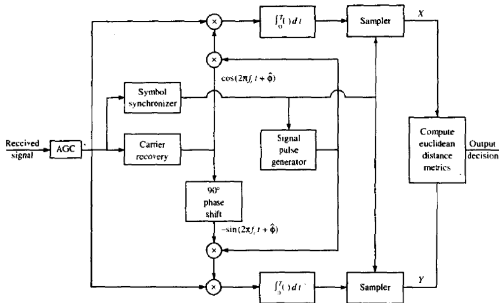
FIGURE 6-1-4 Block diagram of QAM receiver.
