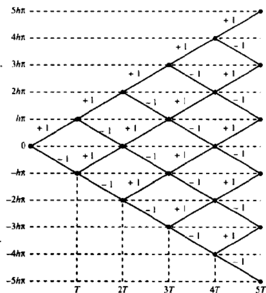
FIGURE 4-3-17 Phase trajectory for binary CPFSK.
