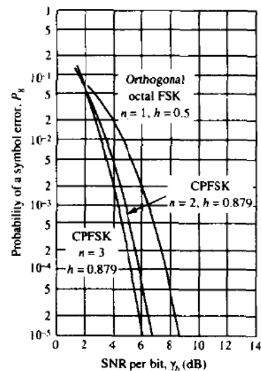
FIGURE 5-3-14 Performance of octal CPFSK with coherent detection.
