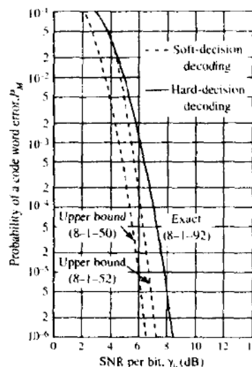
FIGURE 8-1-13 Comparison of soft-decision decoding with hard-decision decoding for the Golay (23, 12) code.
