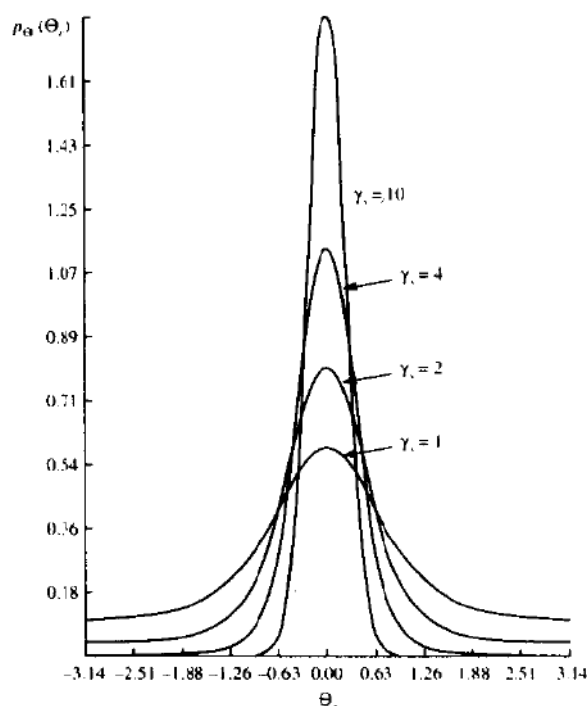
FIGURE 5-2-9 Probability density function p_{\Theta_r}(\Theta_r) for \gamma = 1, 2, 4 and 10 .
