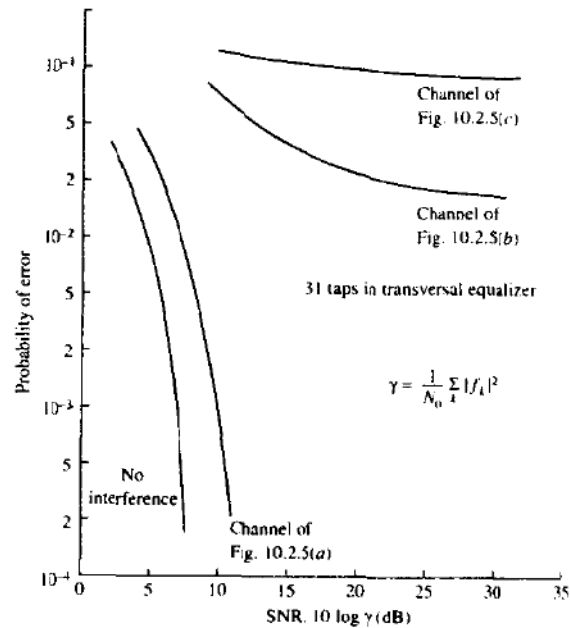
FIGURE 10-2-4 Error rate performance of linear MSE equalizer.
