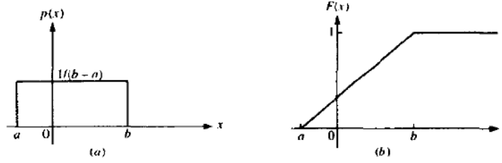
FIGURE 2-1-7 The pdf and cdf of a uniformly distributed random variable.
