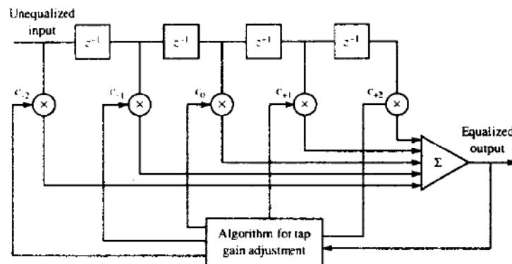
FIGURE 10-2-1 Linear transversal filter.
