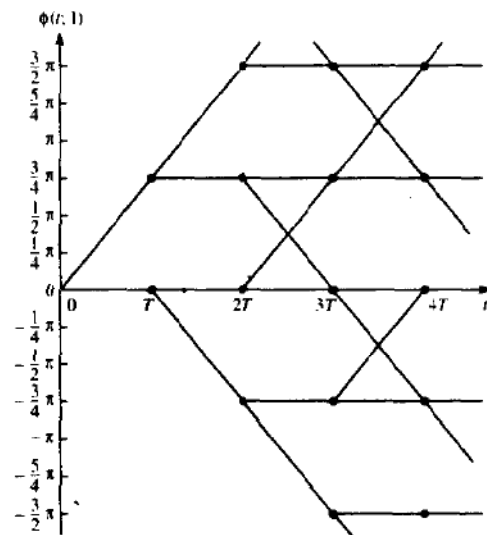
FIGURE 5-3-3 Phase tree for L = 2 partial response CPM with h = 3/4 .
