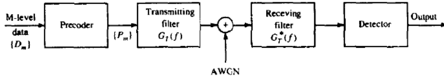
FIGURE 9-3-1 Block diagram of modulator and demodulator for partial-response signals.
