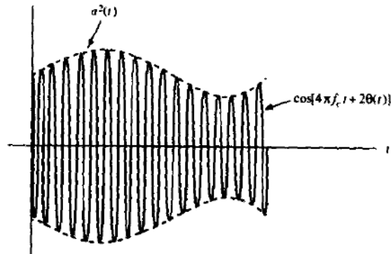
FIGURE 4-1-2 The signal a^2(t) \cos[4\pi f_c t + 2\theta(t)] .
