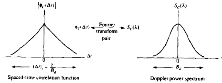
FIGURE 14-1-4 Relationship between \phi_c(\Delta t) and S_c(\lambda) .
