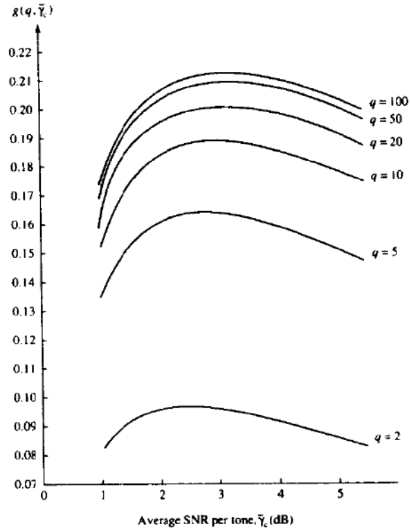
FIGURE 14-6-14 Graph of function g(q, \bar{\gamma}_c) .
