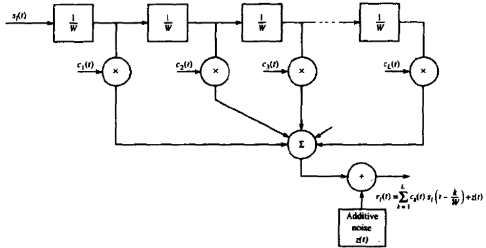
FIGURE 14-5-1 Trapped delay line model of frequency-selective channel.
