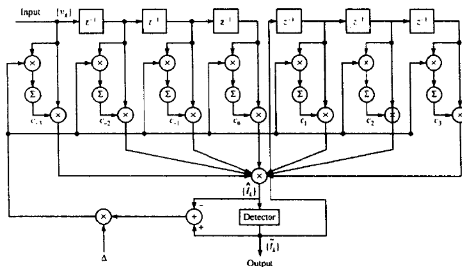
FIGURE 11-2-1 Decision-feedback equalizer.
