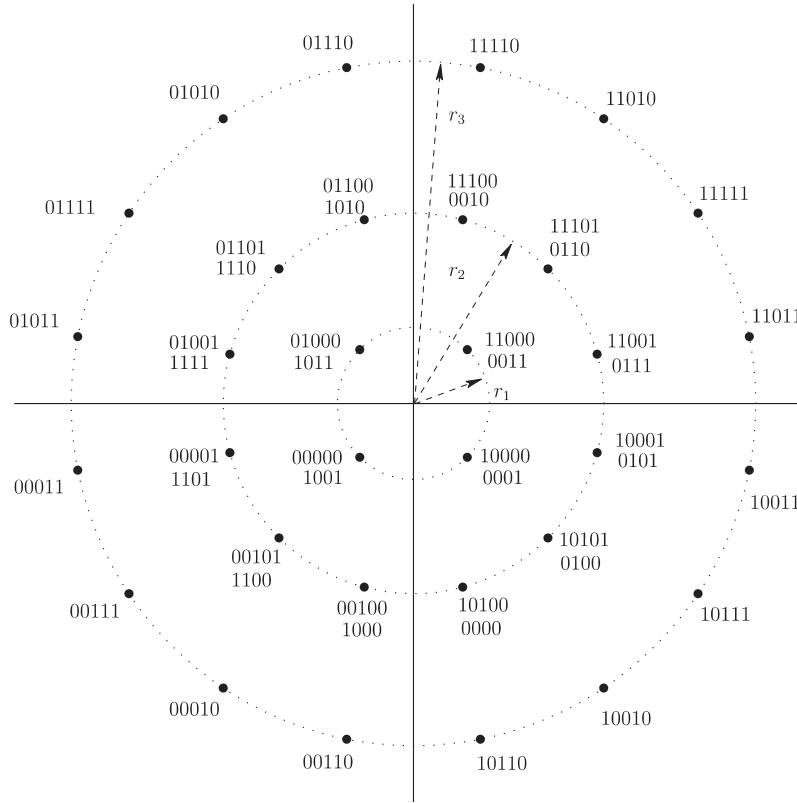
Figure 1. Parametric description and pseudo-Gray mapping of 16 and 32-APSK constellations with n_1 = 4 , n_2 = 12 , \phi_2 = 0 and n_1 = 4 , n_2 = 12 , n_3 = 16 , \phi_2 = 0 , \phi_3 = \pi/16 . For the first two rings: mapping below corresponds to 4 + 12-APSK, mapping above to 4 + 12 + 16-APSK.
