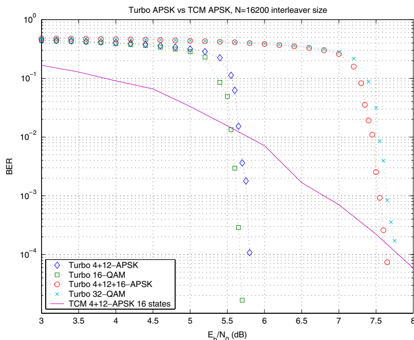
Figure 9. Turbo-coded APSK with N = 16\,200 vs 4 + 12-TCM.
