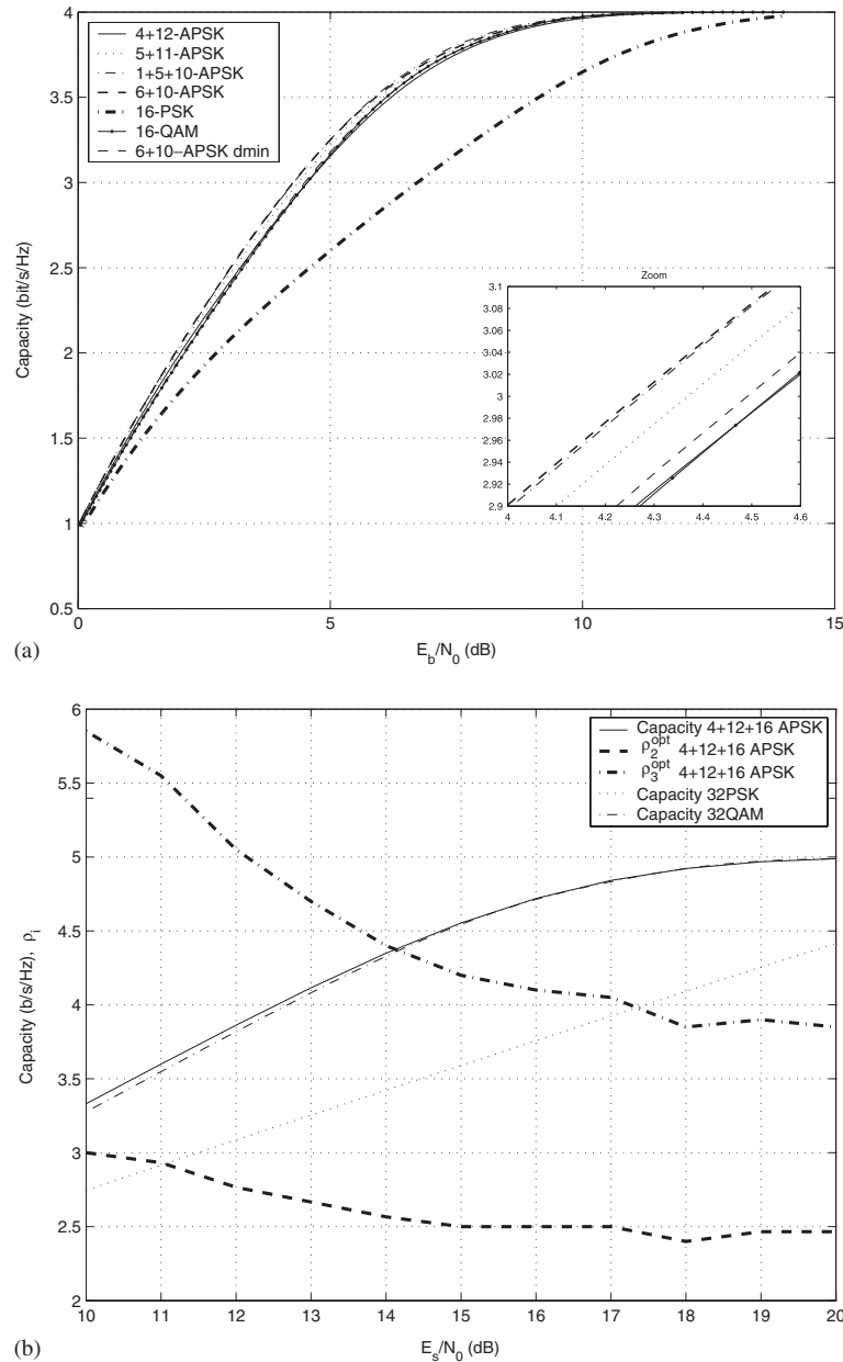
Figure 5. Capacity and \rho^{opt} for the optimized APSK signal constellations vs QAM and PSK: (a) 16-ary constellations (zoom around 3 bps/Hz); and (b) 32-ary constellations.
