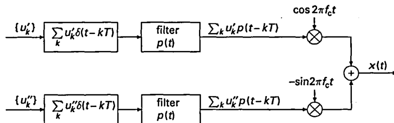
Figure 6.7. DSB-QC modulation.
