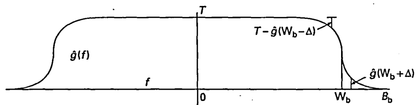
Figure 6.3. Band-edge symmetry illustrated for real \hat{g}(f) . For each \Delta , 0 \leq \Delta \leq W_b , \hat{g}(W_b + \Delta) = T - \hat{g}(W_b - \Delta) . The portion of the curve for f \geq W_b , rotated by 180^\circ around the point (W_b, T/2) , is equal to the portion of the curve for f \leq W_b .
