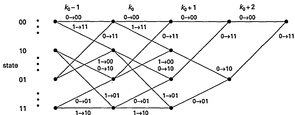
Figure 8.10. Trellis termination.
