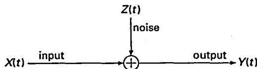
Figure 1.4. Additive white Gaussian noise (AWGN) channel.
