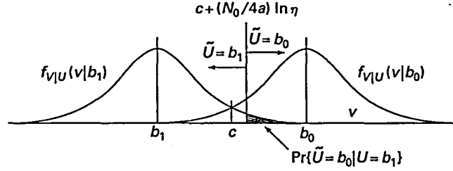
Figure 8.3. Binary hypothesis testing for arbitrary signals, 0 \rightarrow b_0 , 1 \rightarrow b_1 , for b_0 > b_1 . With c = (b_0 + b_1)/2 and a = |b_0 - b_1|/2 , this is the same as Figure 8.2 shifted by c . For b_0 < b_1 , the picture must be reversed, but the answer is the same.
