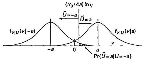
Figure 8.2. Binary hypothesis testing for antipodal signals, 0 \rightarrow a , 1 \rightarrow -a . The a-priori probabilities are p_0 and p_1 , the threshold is \eta = p_0/p_1 , and the noise is \mathcal{N}(0, N_0/2) .
