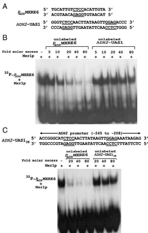
Fig. 8. Analysis of Mxr1p binding to S. cerevisiae ADH2UAS1 by EMSA. (A) Nucleotide sequence of P_{AOX} MXRE6 and ADH2UAS1. The core CYCC motifs are underlined. (B) Competition EMSA was carried out with 0.5 nM radiolabeled probe and 30 nM Mxr1p. Unlabeled P_{AOX} MXRE6 but not ADH2UAS1 competes out binding of Mxr1p to ^{32} P-labeled P_{AOX} MXRE6. (C) Effect of increasing the length of ADH2UAS1 on Mxr1p binding as analyzed by competition EMSA.
