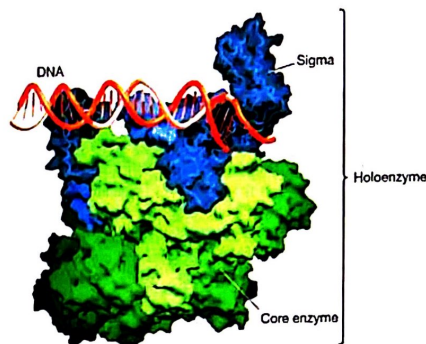
FIGURE 16.2 The Three-Dimensional Structure of RNA Polymerase Bacterial RNA polymerase is a globular enzyme. Sigma is a regulatory component, and the core enzyme contains the active site.
