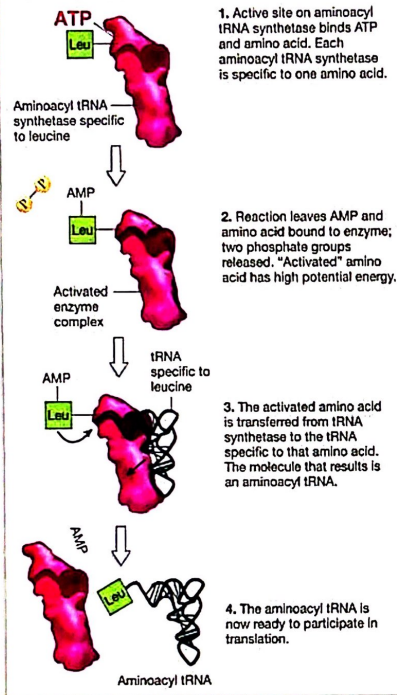
FIGURE 16.10 Aminoacyl tRNA Synthetases Load Amino Acids onto the Appropriate tRNA
