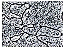
(a) Micrograph of DNA-RNA hybrid
