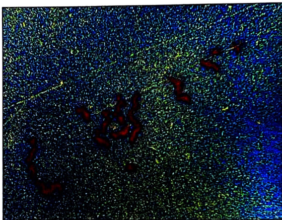
A micrograph showing transcription and translation occurring simultaneously in a bacterial cell. The yellow lines are strands of DNA, and the red structures are ribosomes.
