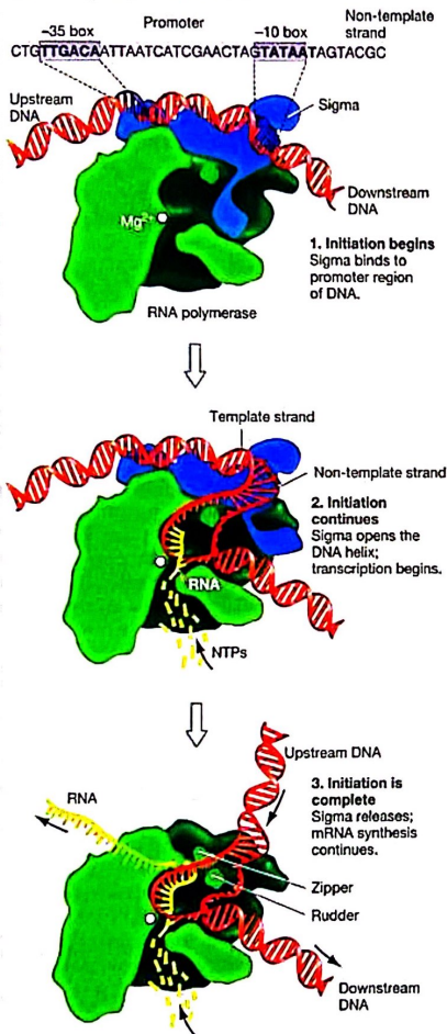
FIGURE 16.3 In Bacteria, Sigma Plays a Key Role in Initiating Transcription
