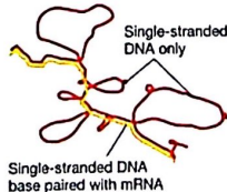
(b) Interpretation of micrograph
