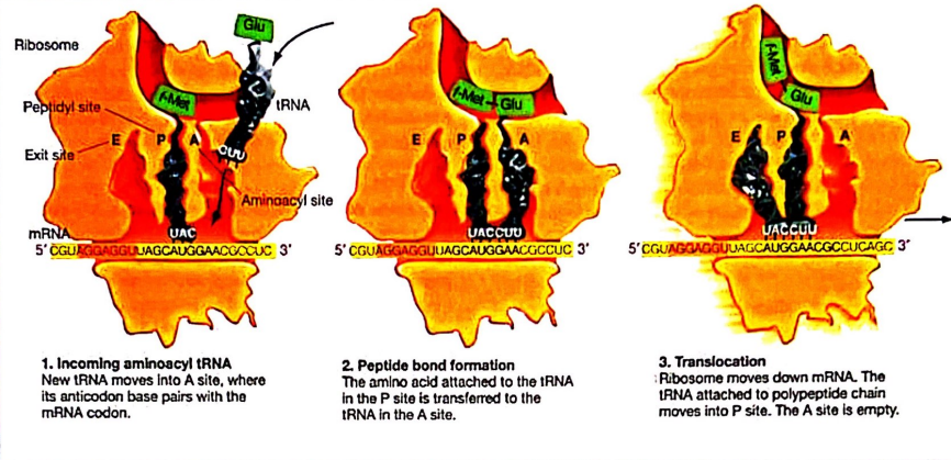
FIGURE 16.15 The Elongation Phase of Translation
