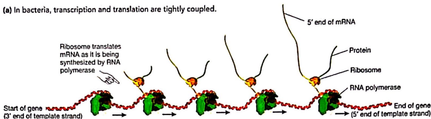
FIGURE 16.8 Transcription and Translation Occur Simultaneously in Bacteria but Not in Eukaryotes
