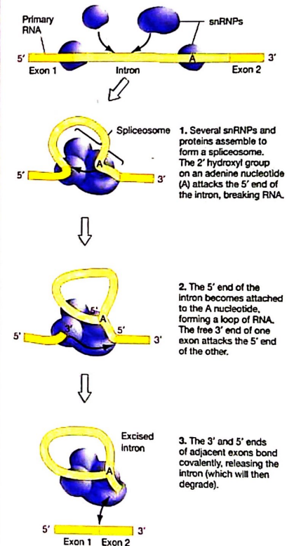
FIGURE 16.6 Introns Are Spliced Out of the Original mRNA (a) RNA polymerase produces a primary RNA transcript that contains exons and introns. Subsequent processing generates a mature transcript. (b) snRNPs are responsible for the splicing reactions that take place in the nucleus of eukaryotes.
