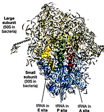
FIGURE 16.13 The Structure of the Ribosome
