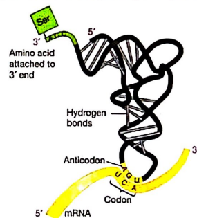
(c) Revised model incorporating tertiary structure of tRNA
