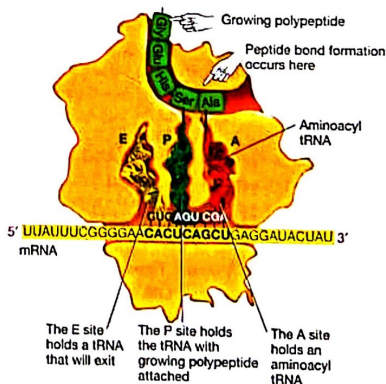
(b) Diagram of ribosome during translation
