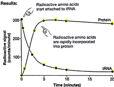
FIGURE 16.11 Experimental Evidence That Amino Acids Are Transferred from tRNAs to Proteins
