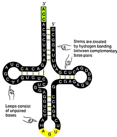
(a) Secondary structure of tRNA
