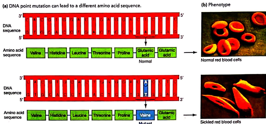
FIGURE 16.19 Sickle-Cell Disease Results from a Point Mutation in the Gene for Hemoglobin (a) These normal and mutant genes that code for hemoglobin differ by a single nucleotide. The sequences shown are just a small portion of the gene. (b) The mutation in part (a) changes the primary sequence of the gene product. The change in amino acid sequence causes hemoglobin molecules to crystallize when oxygen levels in the blood are low. As a result, red blood cells sickle and get stuck in small blood vessels. EXERCISE The mRNA codon GUG specifies the valine at the start (left) of this protein. Label the template strand and the non-template strand of DNA, and indicate their 5' and 3' ends.
