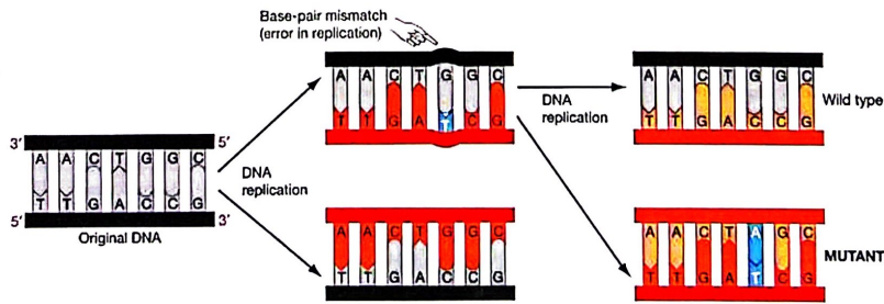
FIGURE 16.18 Unrepaired Mistakes in DNA Synthesis Lead to Point Mutations
