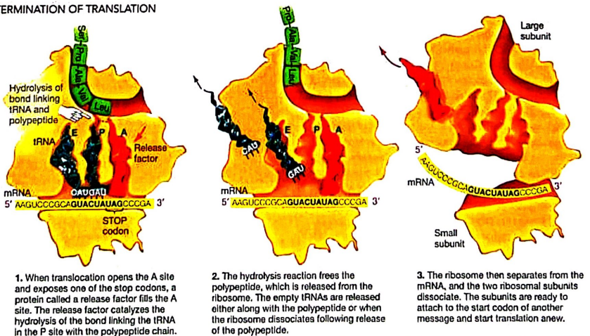
FIGURE 16.17 The Termination Phase of Translation
