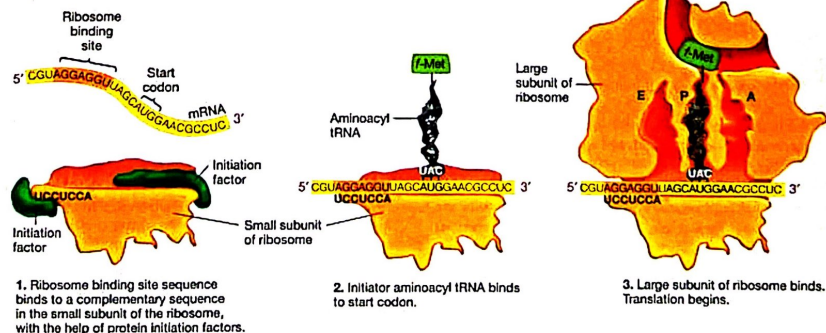
FIGURE 16.14 The Initiation Phase of Translation in Bacteria
